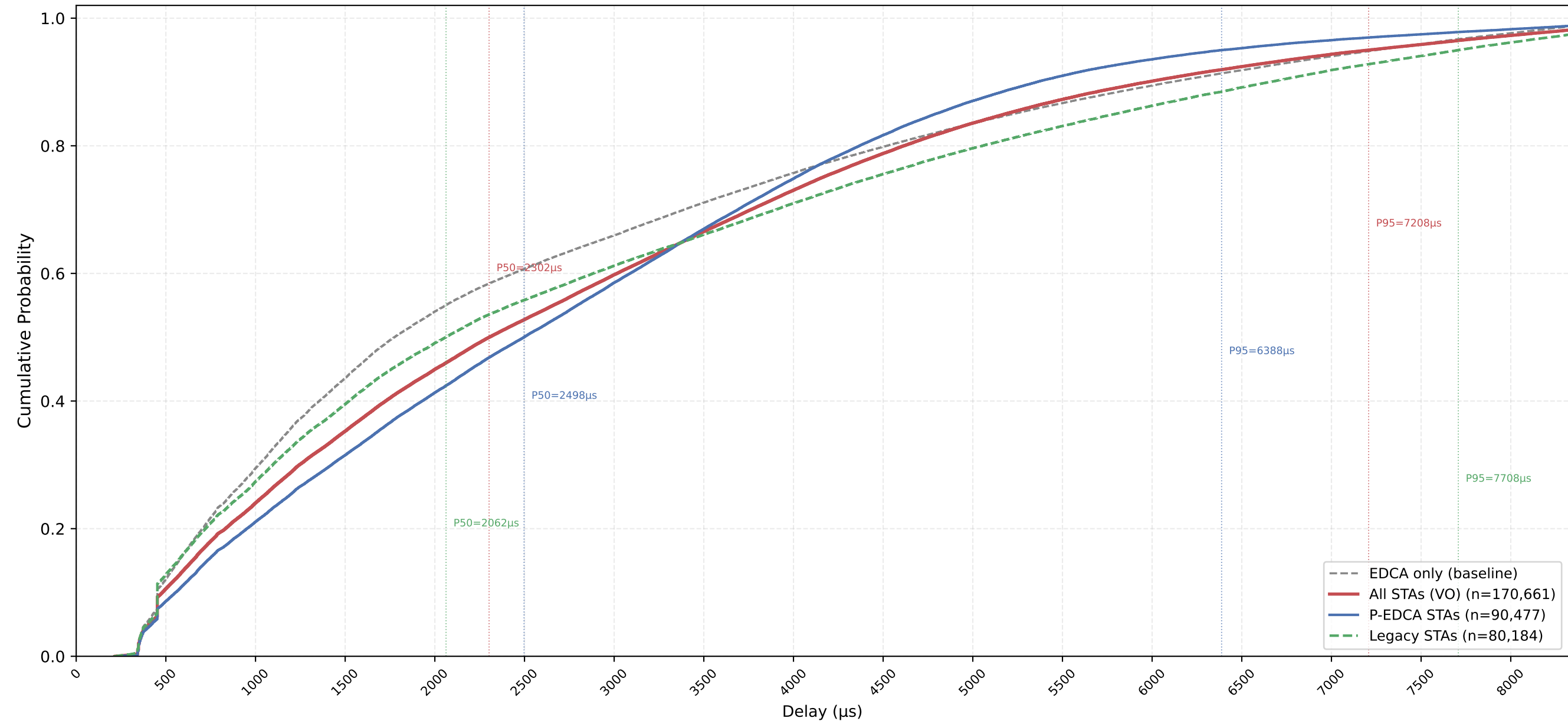
VO Delay CDF — P-EDCA / Legacy / All | CWds=0 × QSRC=2 × PSRC=1 nSta=30, nPedca=15/30, 1Mbps, avg of 10 runs
