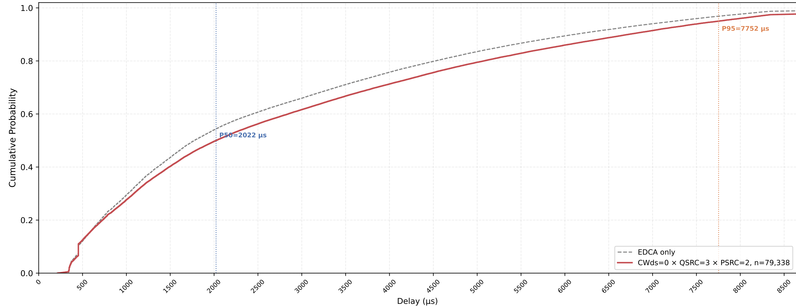
Legacy STA VO Delay CDF — CWds=0 × QSRC=3 × PSRC=2 nSta=30, nPedca=15, 1Mbps, avg of 10 runs
