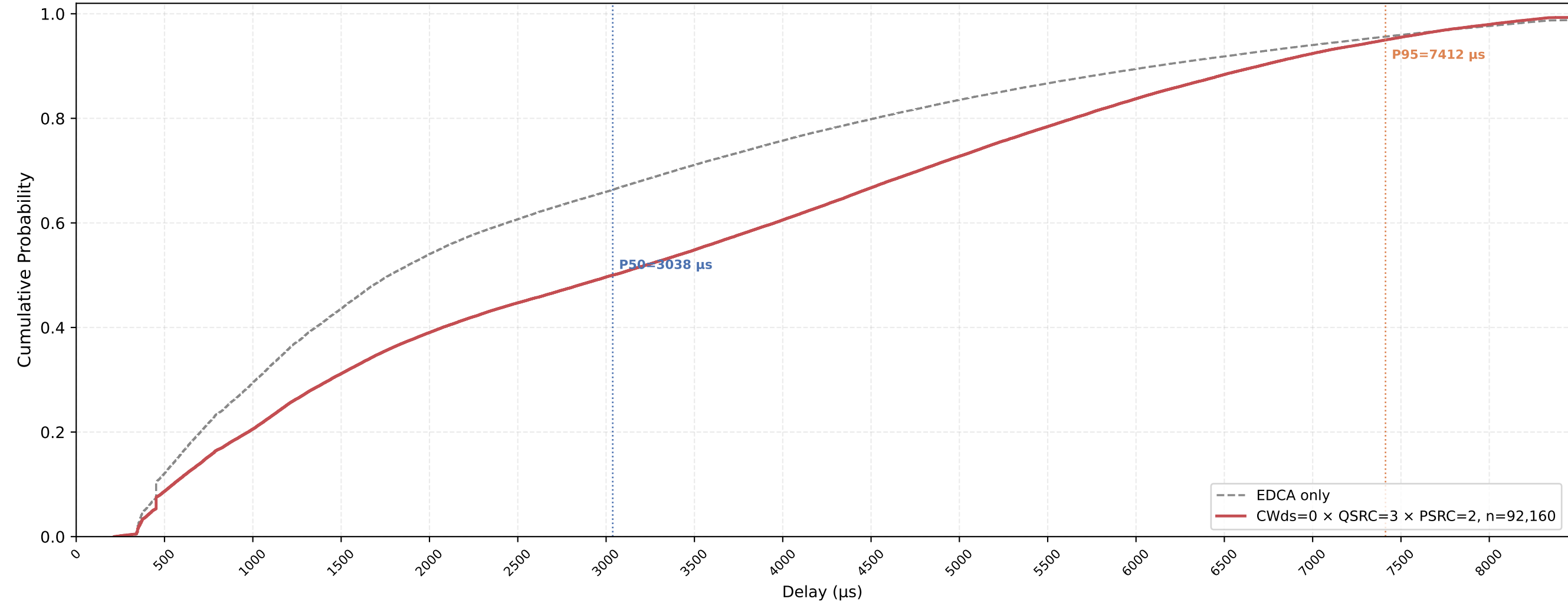
P-EDCA STA VO Delay CDF — CWds=0 × QSRC=3 × PSRC=2 nSta=30, nPedca=15, 1Mbps, avg of 10 runs
