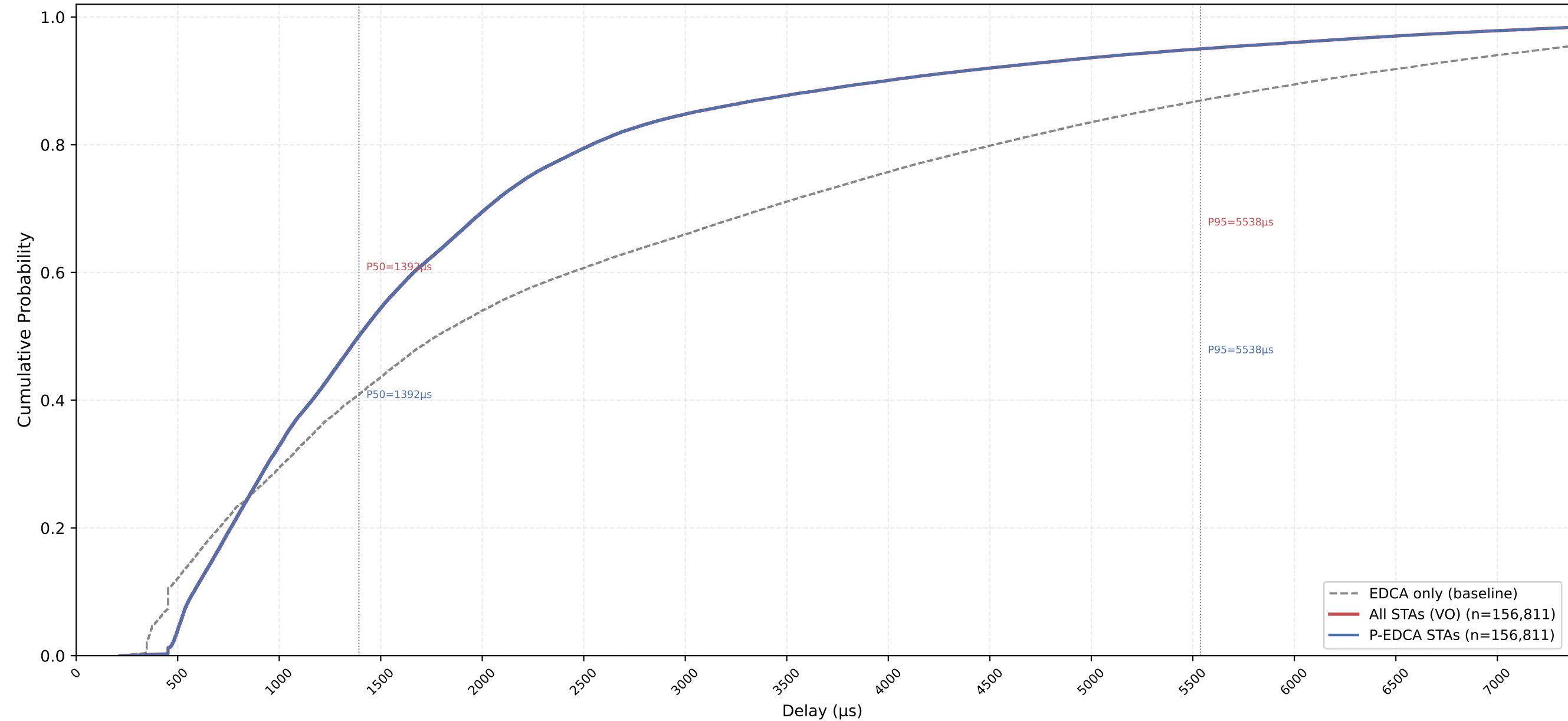
VO Delay CDF — P-EDCA / Legacy / All | CWds=1 × QSRC=0 × PSRC=1 nSta=30, nPedca=30/30, 1Mbps, avg of 10 runs
