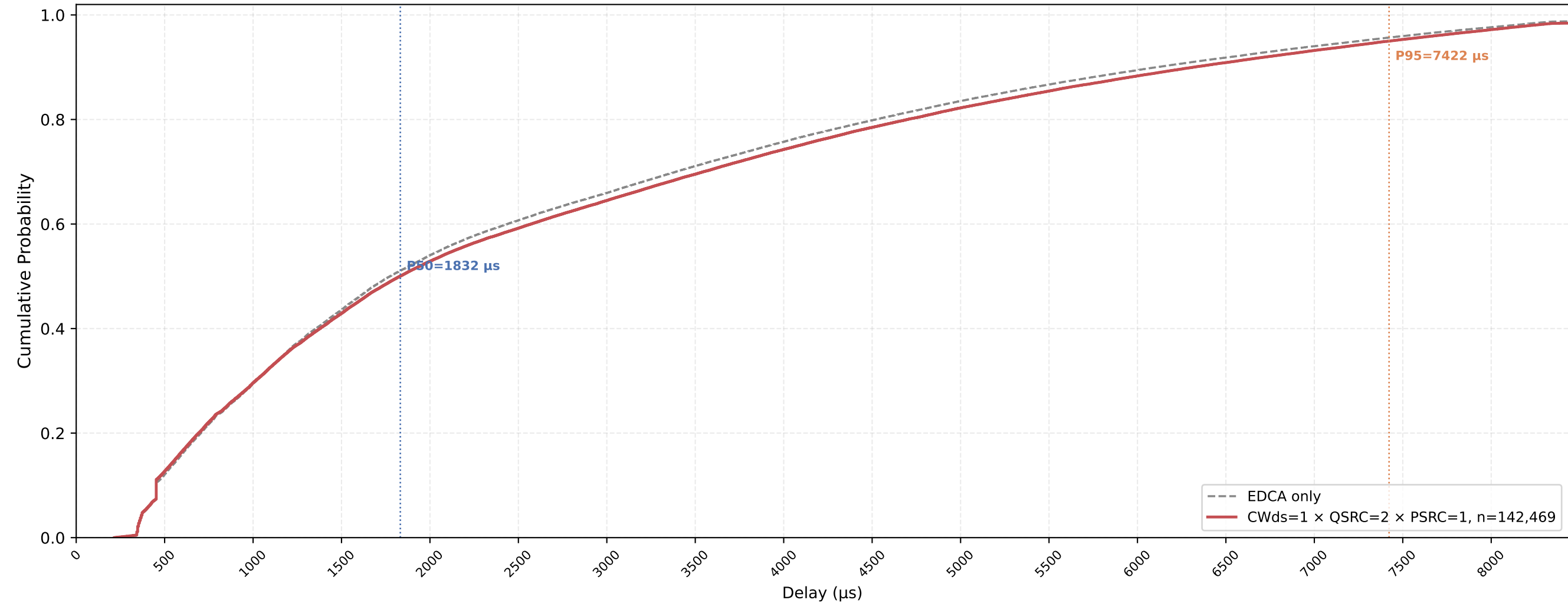
Legacy STA VO Delay CDF — CWds=1 × QSRC=2 × PSRC=1 nSta=30, nPedca=5, 1Mbps, avg of 10 runs
