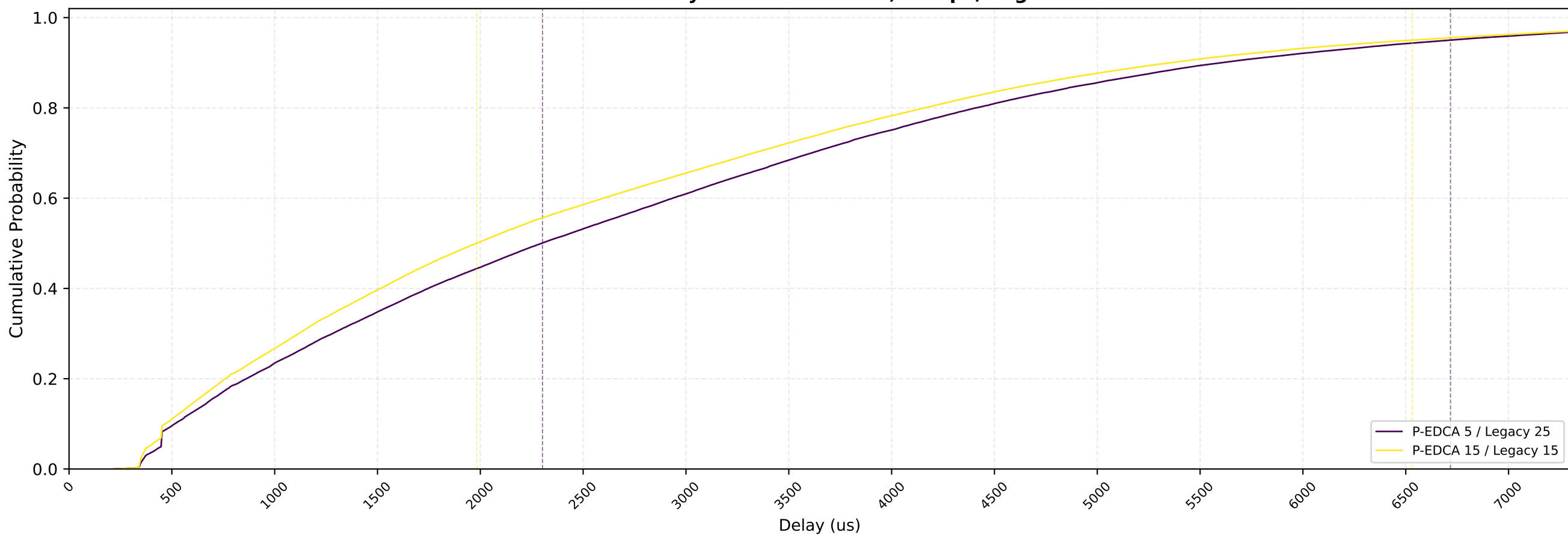
P-EDCA STAs Delay CDF — nSta=30, 1Mbps, avg of 10 runs
