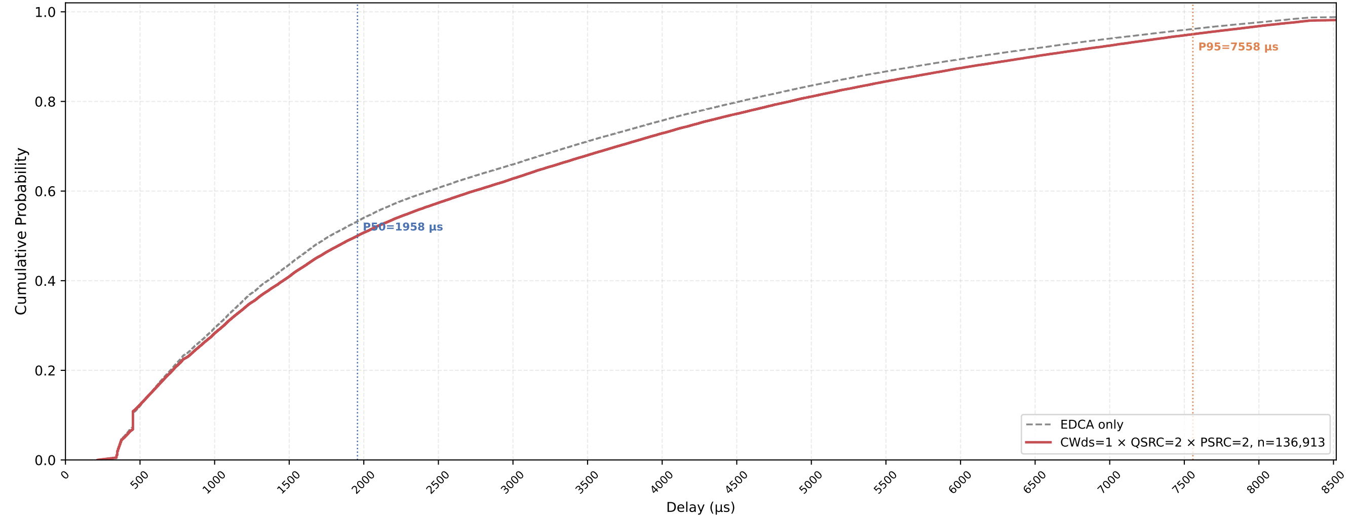
Legacy STA VO Delay CDF — CWds=1 × QSRC=2 × PSRC=2 nSta=30, nPedca=5, 1Mbps, avg of 10 runs
