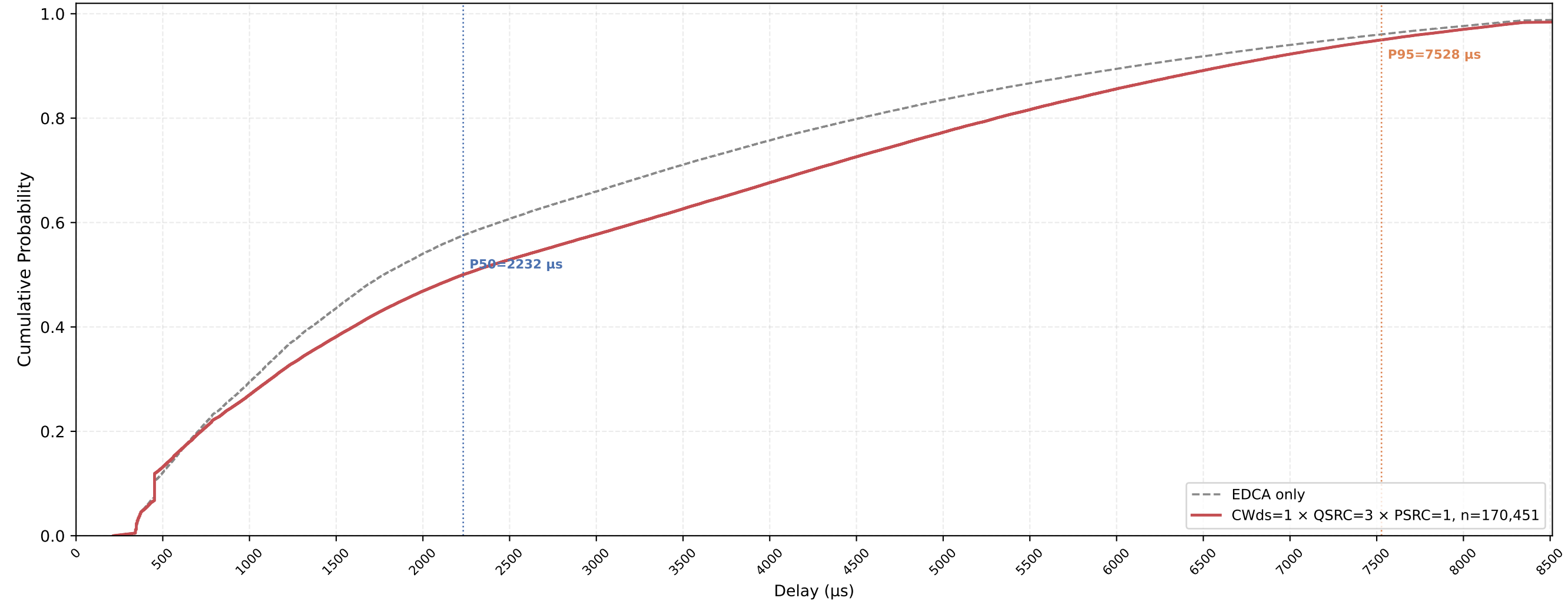
P-EDCA STA VO Delay CDF — CWds=1 × QSRC=3 × PSRC=1 nSta=30, nPedca=30, 1Mbps, avg of 10 runs
