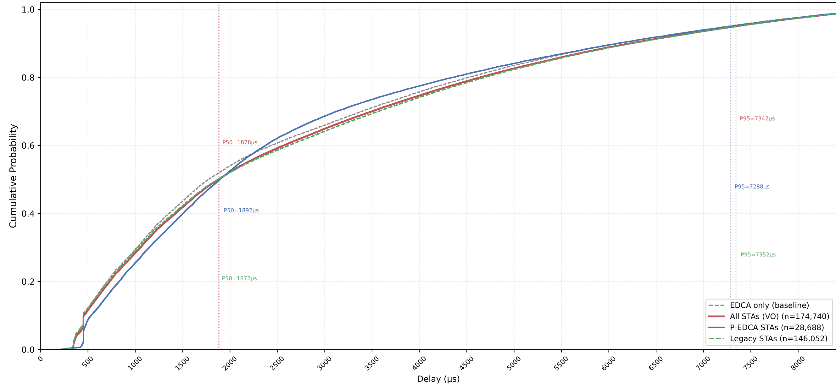
VO Delay CDF — P-EDCA / Legacy / All | CWds=0 × QSRC=0 × PSRC=1 nSta=30, nPedca=5/30, 1Mbps, avg of 10 runs
