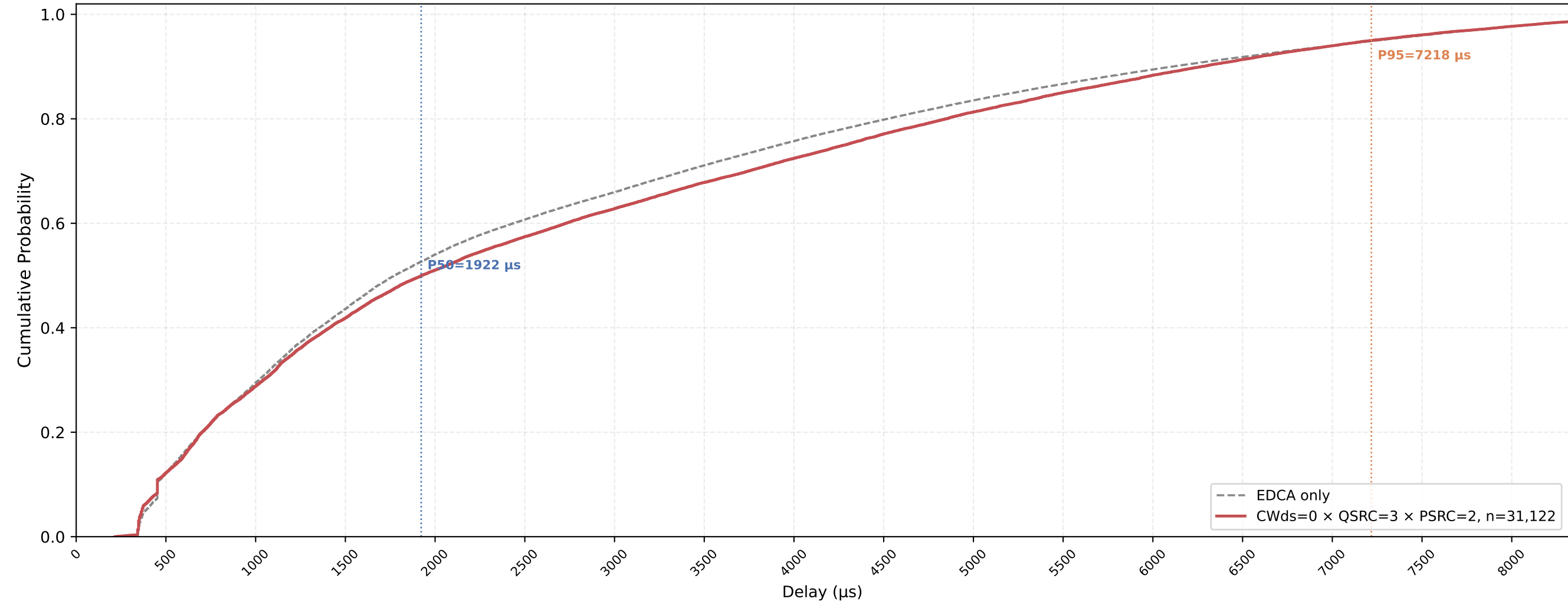
P-EDCA STA VO Delay CDF — CWds=0 × QSRC=3 × PSRC=2 nSta=30, nPedca=5, 1Mbps, avg of 10 runs
