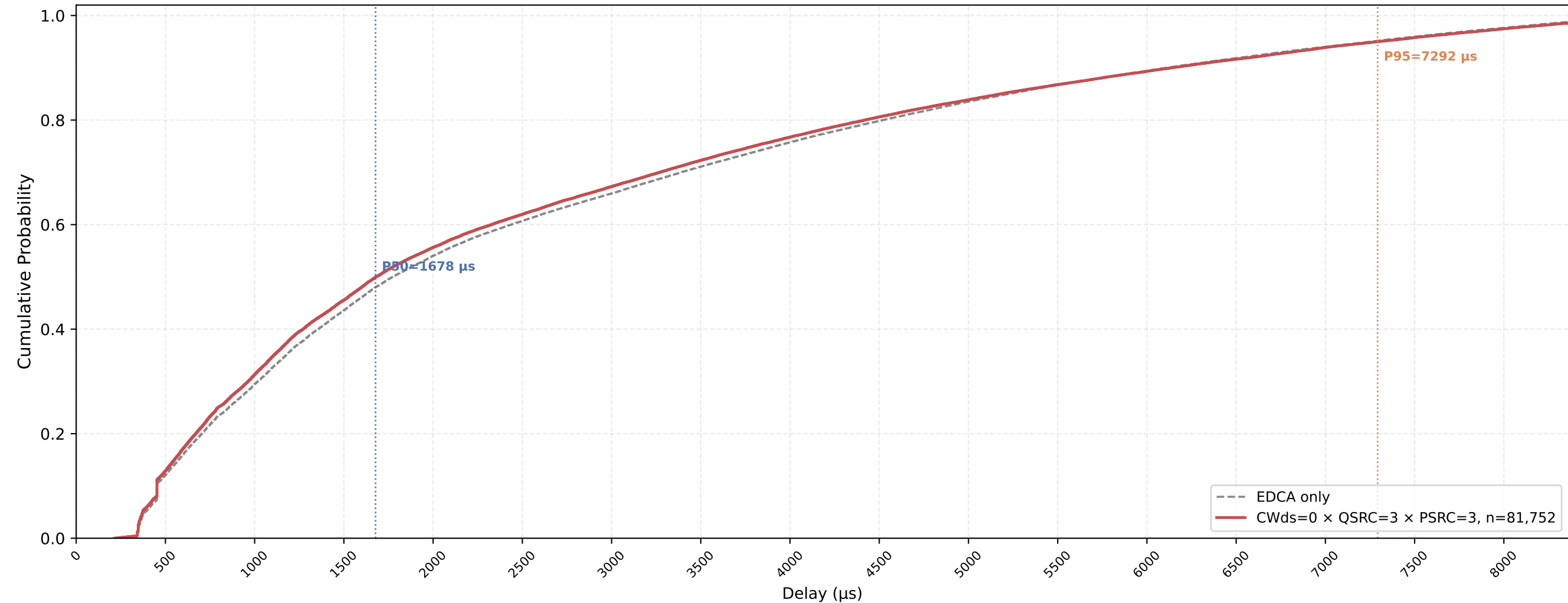
Legacy STA VO Delay CDF — CWds=0 × QSRC=3 × PSRC=3 nSta=30, nPedca=15, 1Mbps, avg of 10 runs
