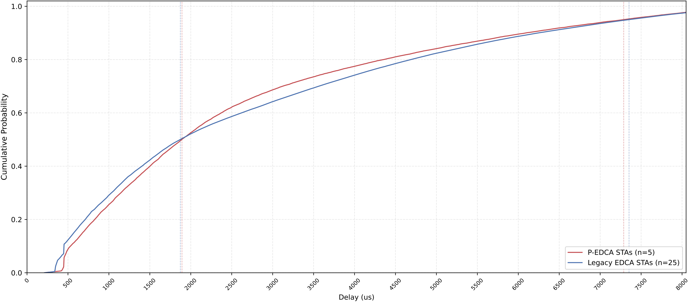
P-EDCA vs Legacy Delay CDF — n_pedca=5, n_legacy=25, nSta=30, 1Mbps, avg of 10 runs
