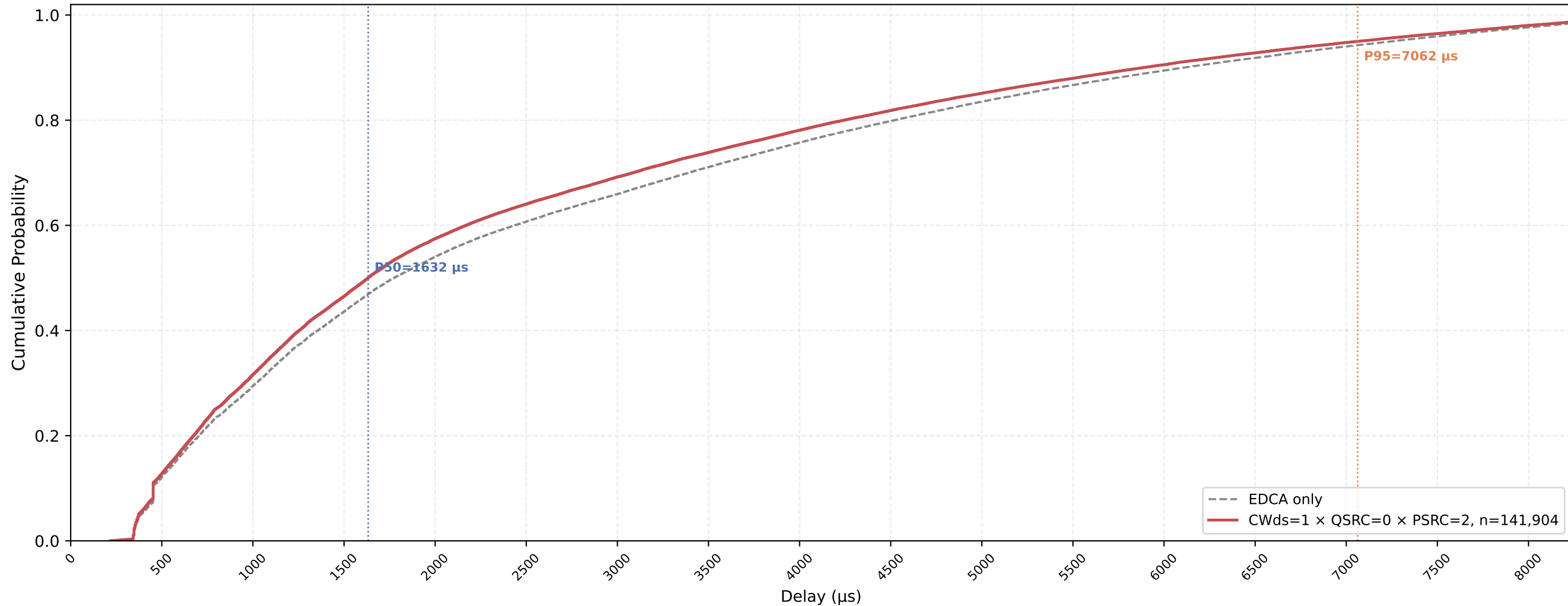
Legacy STA VO Delay CDF — CWds=1 × QSRC=0 × PSRC=2 nSta=30, nPedca=5, 1Mbps, avg of 10 runs
