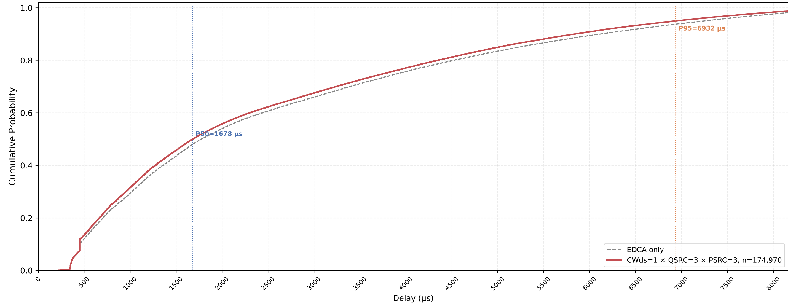
VO (all STAs) Delay CDF — CWds=1 × QSRC=3 × PSRC=3 nSta=30, nPedca=30, 1Mbps, avg of 10 runs
