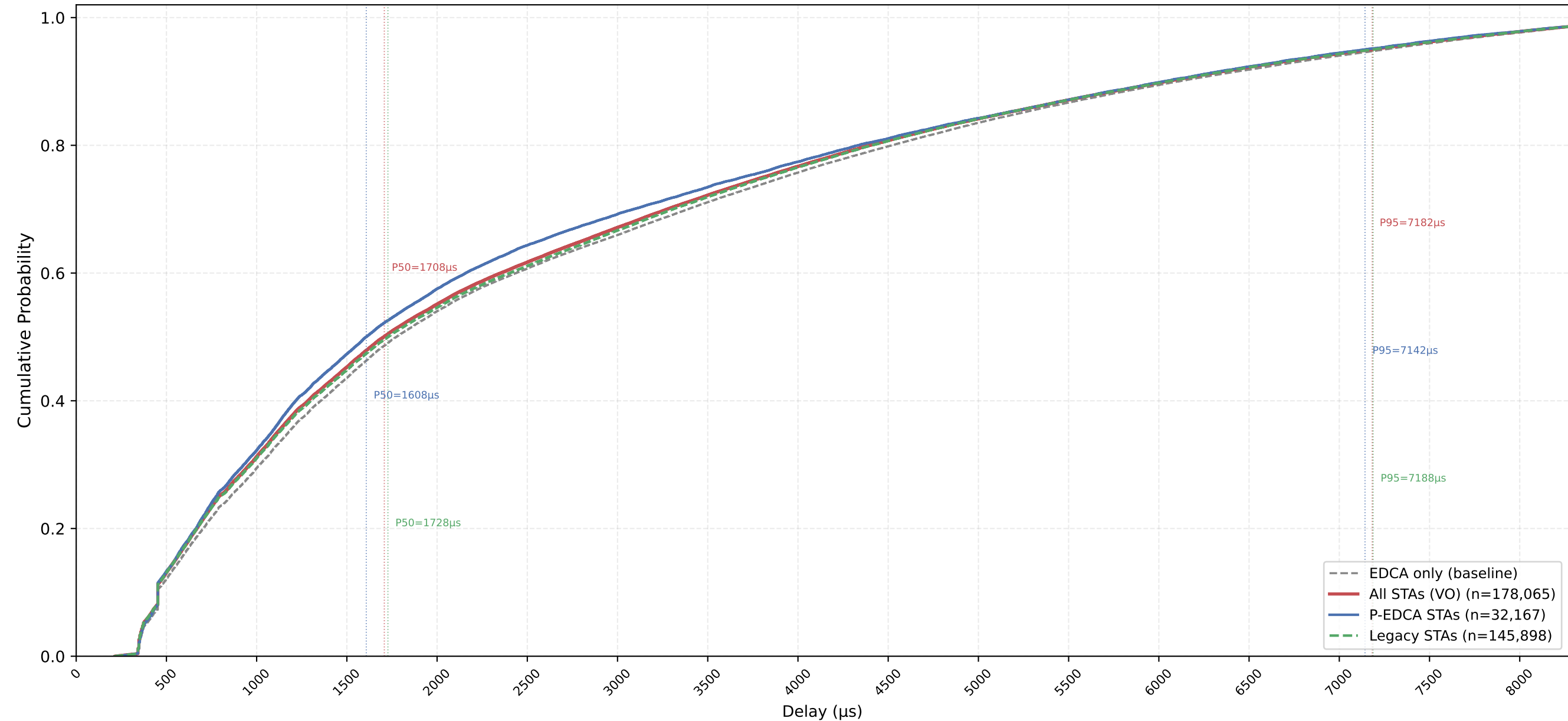
VO Delay CDF — P-EDCA / Legacy / All | CWds=1 × QSRC=4 × PSRC=1 nSta=30, nPedca=5/30, 1Mbps, avg of 10 runs
