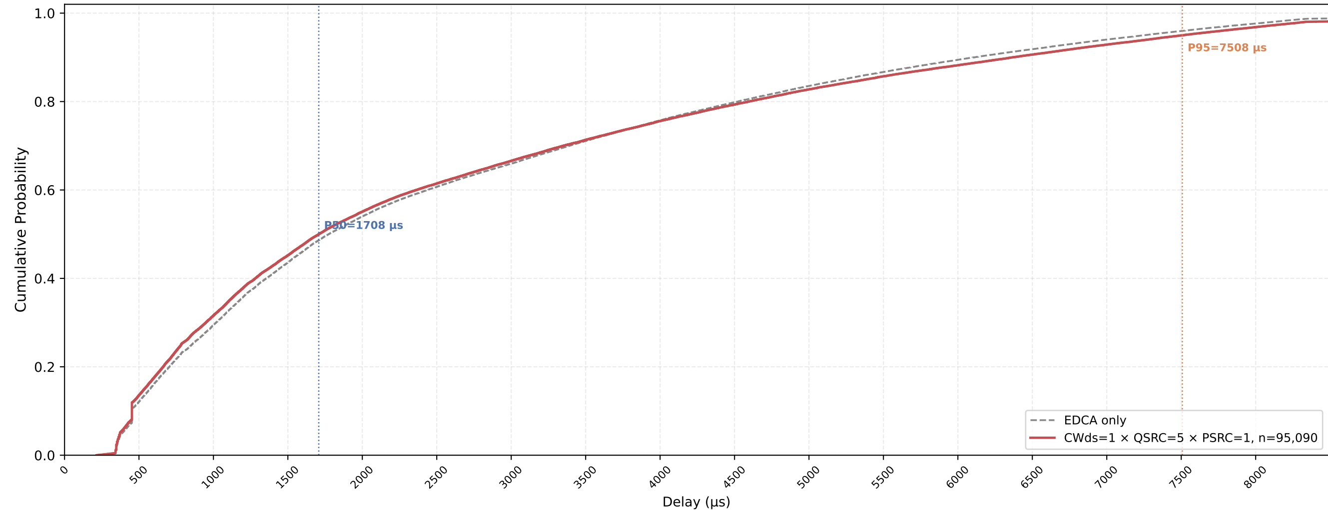
P-EDCA STA VO Delay CDF — CWds=1 × QSRC=5 × PSRC=1 nSta=30, nPedca=15, 1Mbps, avg of 10 runs
