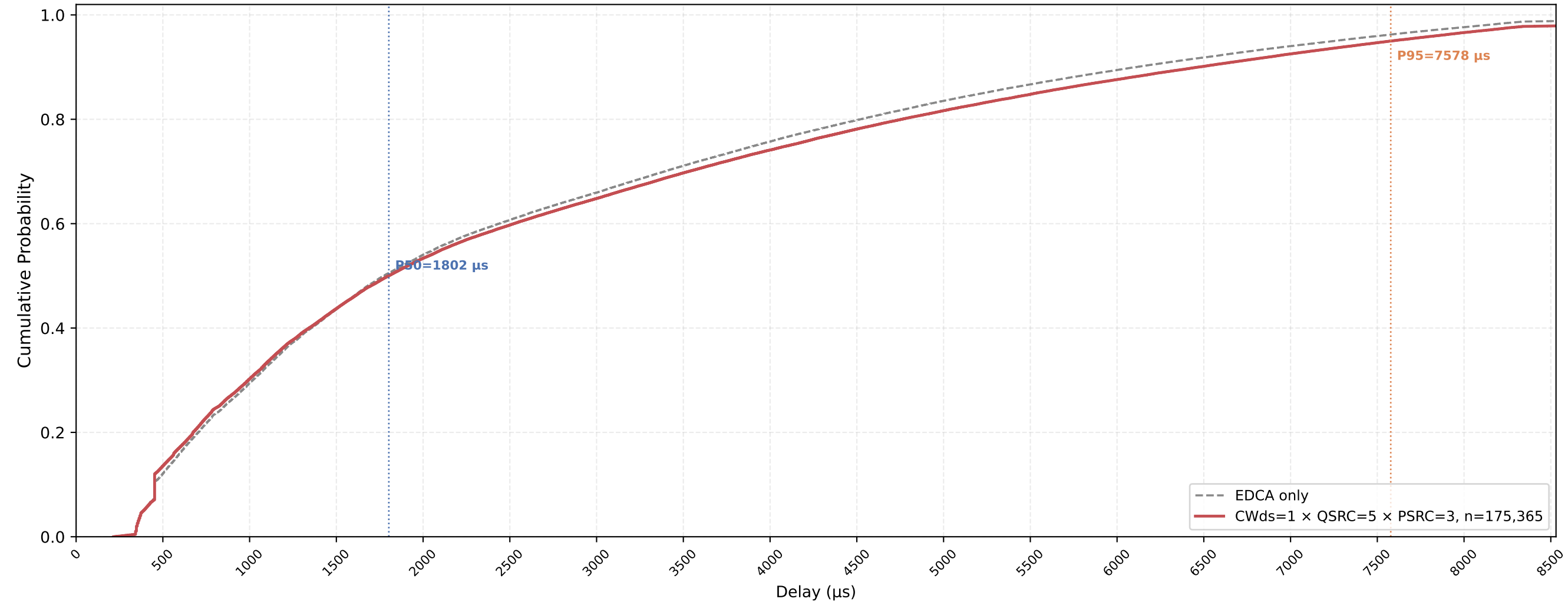
VO (all STAs) Delay CDF — CWds=1 × QSRC=5 × PSRC=3 nSta=30, nPedca=30, 1Mbps, avg of 10 runs
