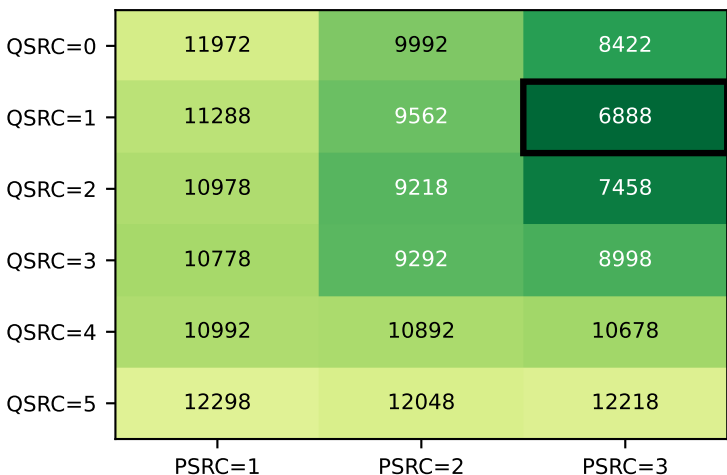
P-EDCA STA VO Delay — P99 Dual-DS (2x DS-CTS) (nSta=30, 1Mbps, black box = best in panel) colour scale 6888-19798 shared across mono-DS & dual-DS — panels are directly comparable
