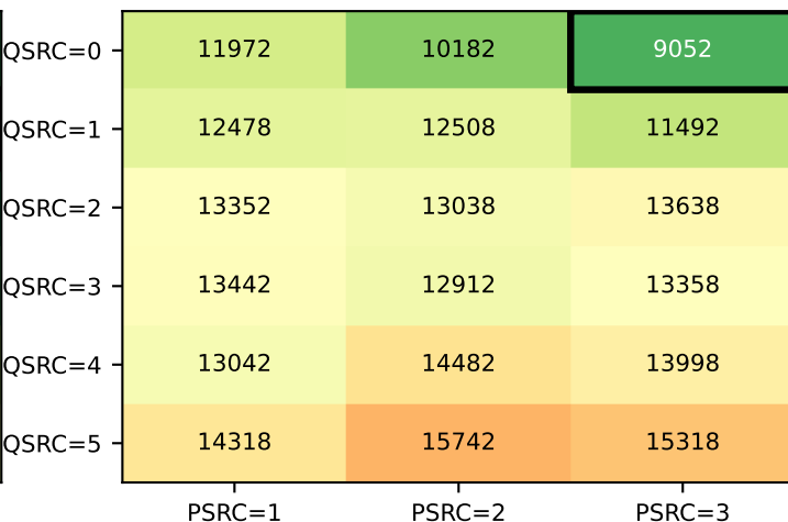
P-EDCA STA VO Delay — P99 Dual-DS (2x DS-CTS) (nSta=30, 1Mbps, black box = best in panel) colour scale 6888-19798 shared across mono-DS & dual-DS — panels are directly comparable
