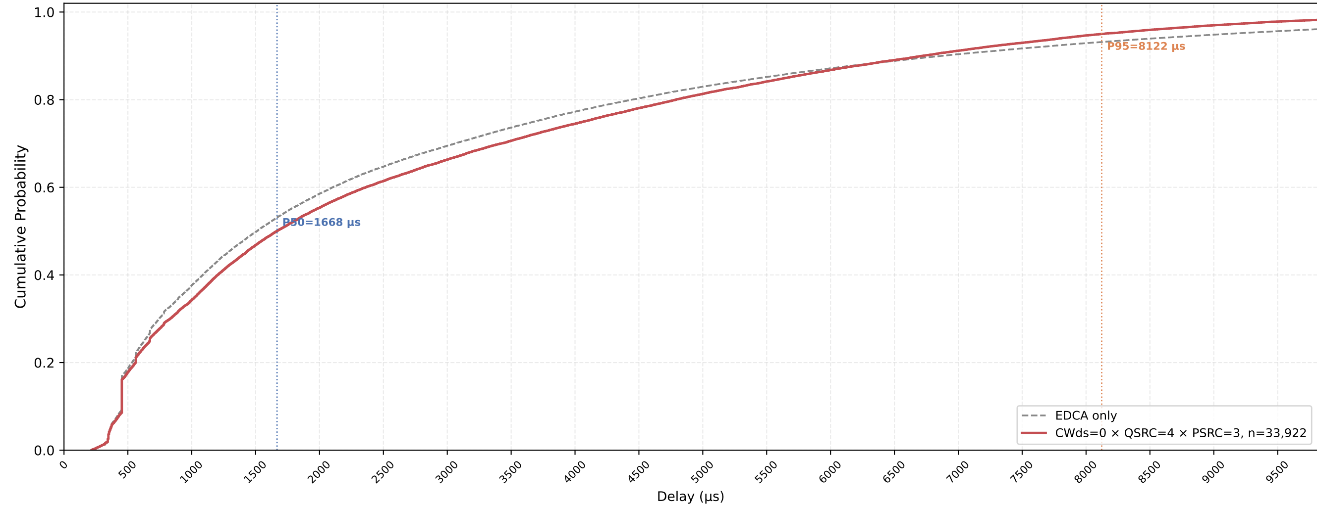
P-EDCA STA VO Delay CDF — CWds=0 × QSRC=4 × PSRC=3 nSta=30, nPedca=5, 1Mbps, avg of 10 runs
