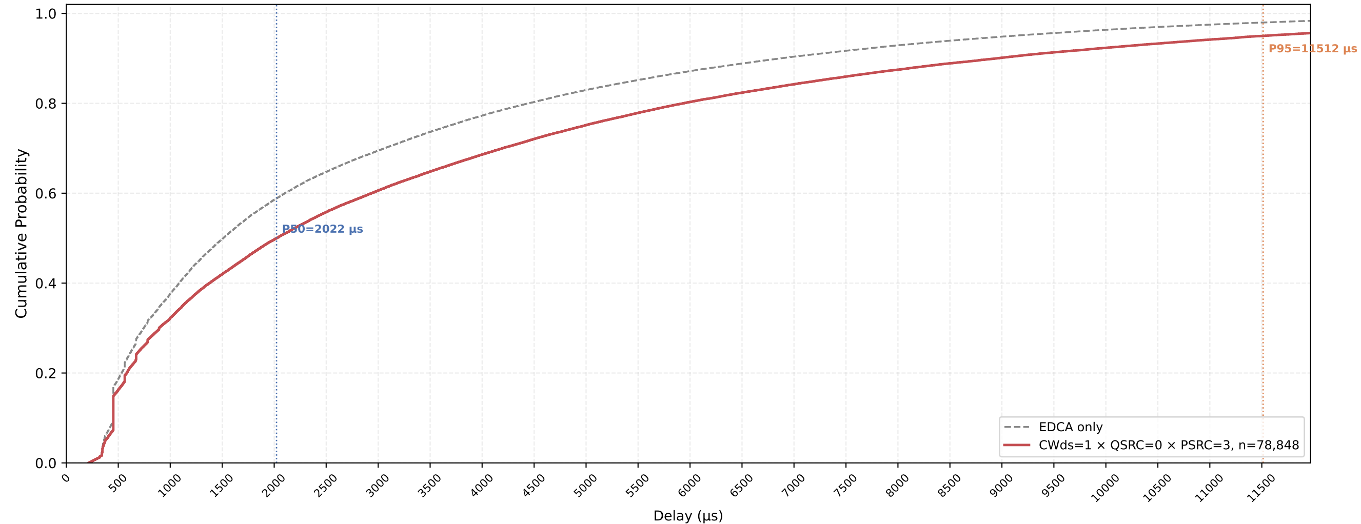
Legacy STA VO Delay CDF — CWds=1 × QSRC=0 × PSRC=3 nSta=30, nPedca=15, 1Mbps, avg of 10 runs
