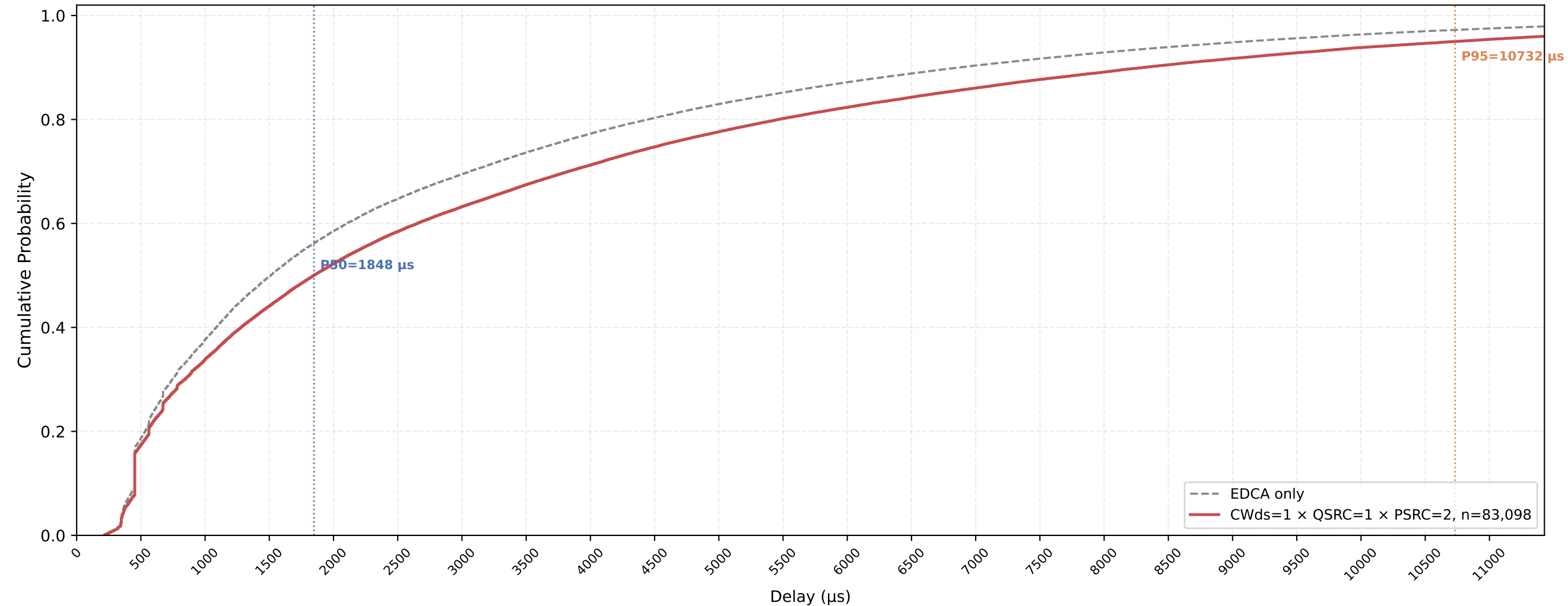
Legacy STA VO Delay CDF — CWds=1 × QSRC=1 × PSRC=2 nSta=30, nPedca=15, 1Mbps, avg of 10 runs
