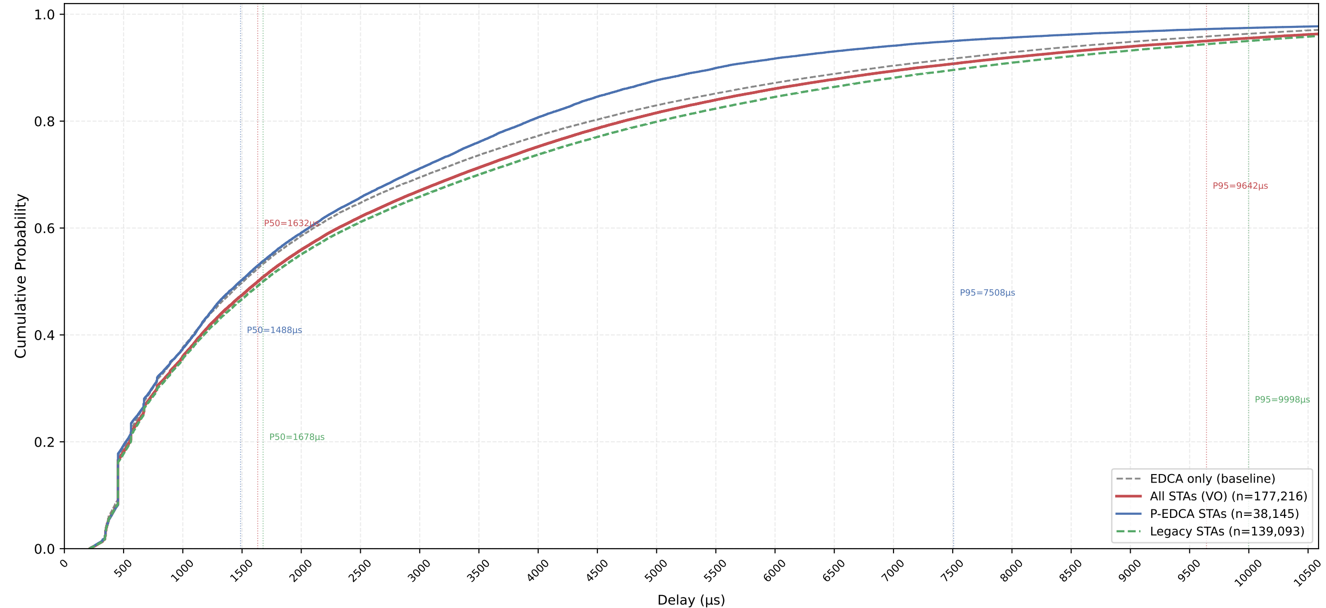
VO Delay CDF — P-EDCA / Legacy / All | CWds=1 × QSRC=2 × PSRC=3 nSta=30, nPedca=5/30, 1Mbps, avg of 10 runs
