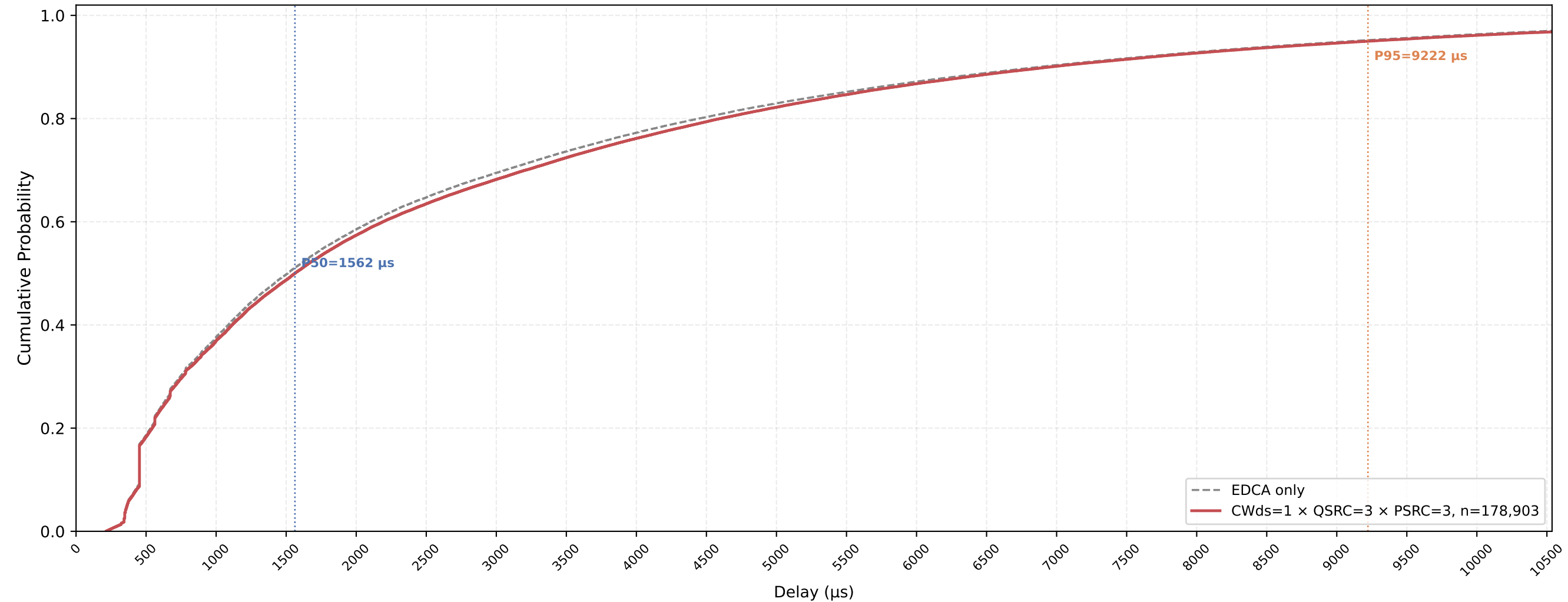
VO (all STAs) Delay CDF — CWds=1 × QSRC=3 × PSRC=3 nSta=30, nPedca=5, 1Mbps, avg of 10 runs
