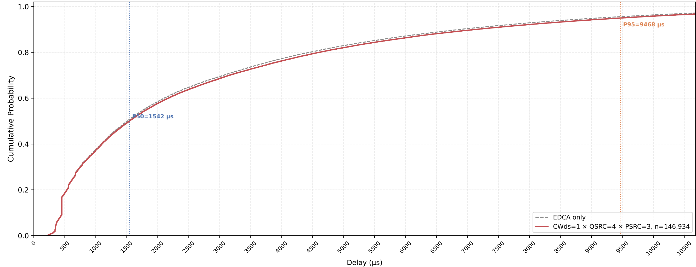
Legacy STA VO Delay CDF — CWds=1 × QSRC=4 × PSRC=3 nSta=30, nPedca=5, 1Mbps, avg of 10 runs
