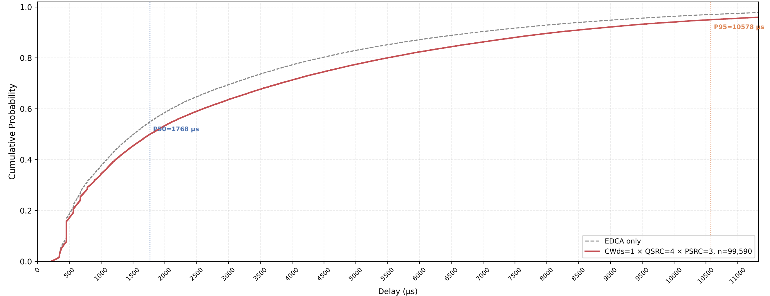
P-EDCA STA VO Delay CDF — CWds=1 × QSRC=4 × PSRC=3 nSta=30, nPedca=15, 1Mbps, avg of 10 runs
