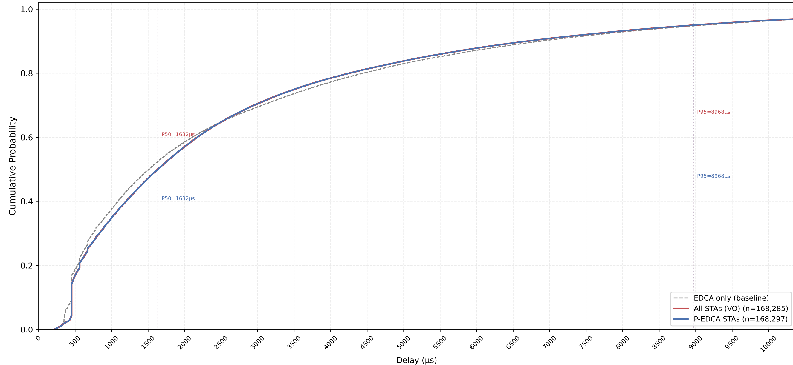
VO Delay CDF — P-EDCA / Legacy / All | CWds=0 × QSRC=0 × PSRC=1 nSta=30, nPedca=30/30, 1Mbps, avg of 10 runs
