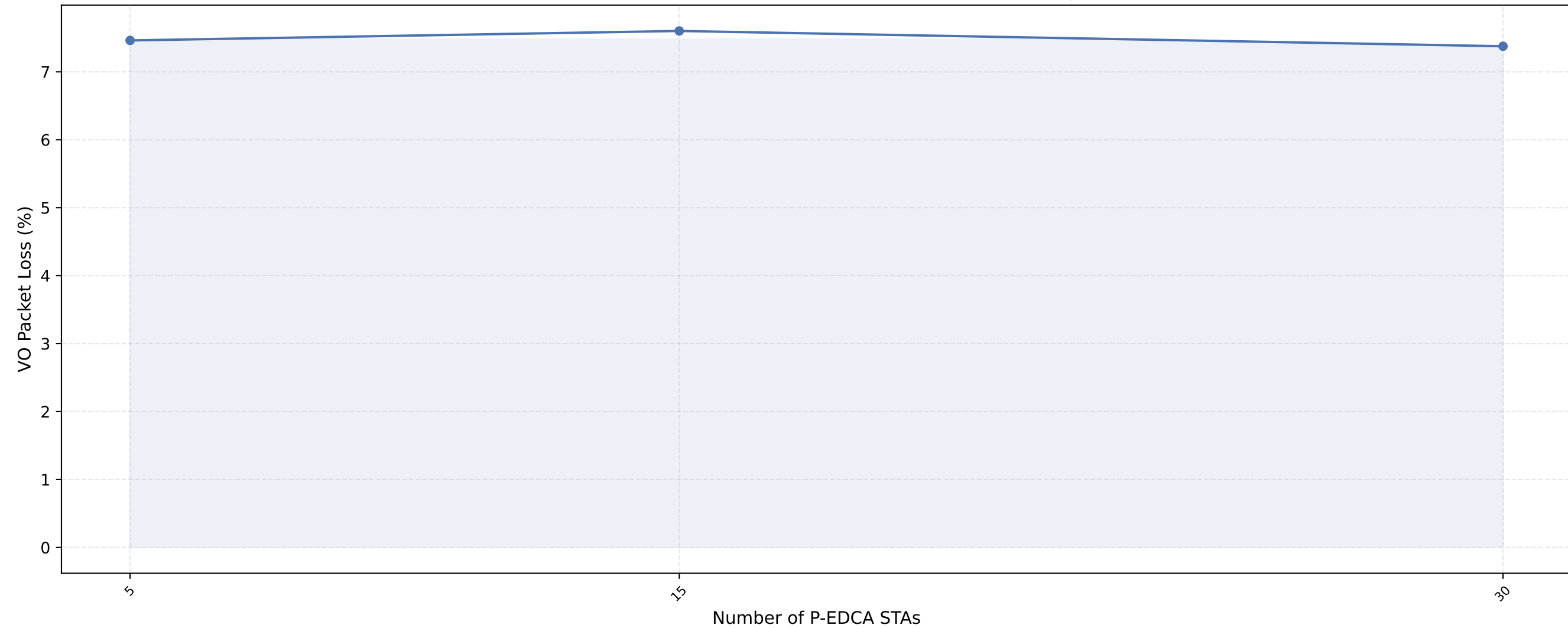
VO Packet Loss vs P-EDCA STAs — nSta=30, 1Mbps (avg of 10 runs)
