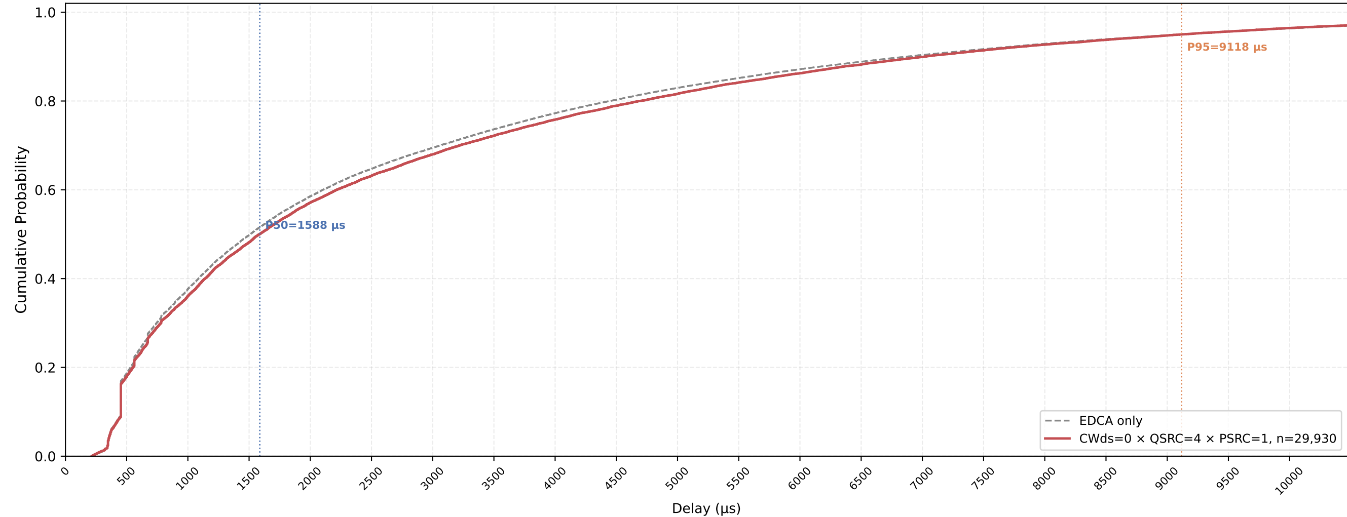
P-EDCA STA VO Delay CDF — CWds=0 × QSRC=4 × PSRC=1 nSta=30, nPedca=5, 1Mbps, avg of 10 runs
