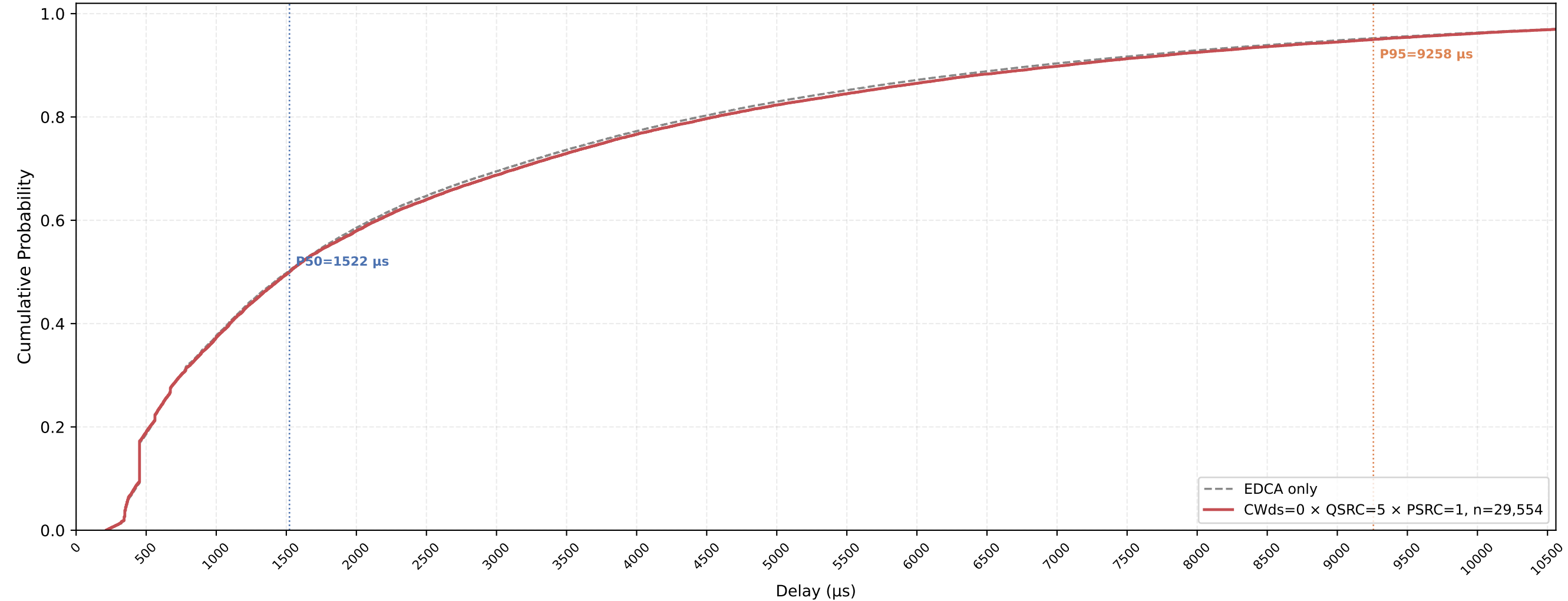
P-EDCA STA VO Delay CDF — CWds=0 × QSRC=5 × PSRC=1 nSta=30, nPedca=5, 1Mbps, avg of 10 runs
