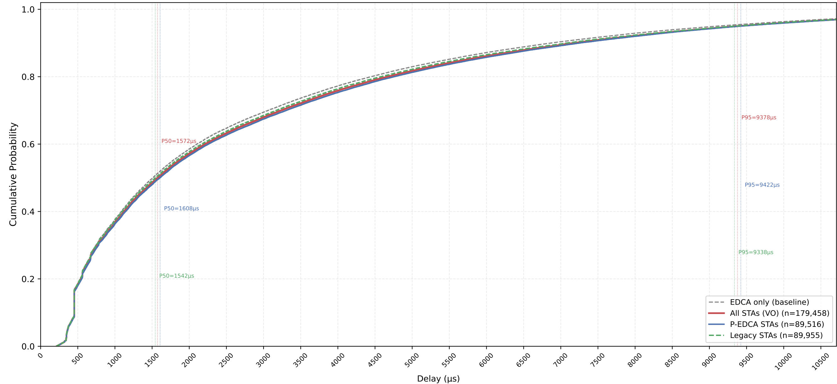
VO Delay CDF — P-EDCA / Legacy / All | CWds=0 × QSRC=5 × PSRC=2 nSta=30, nPedca=15/30, 1Mbps, avg of 10 runs
