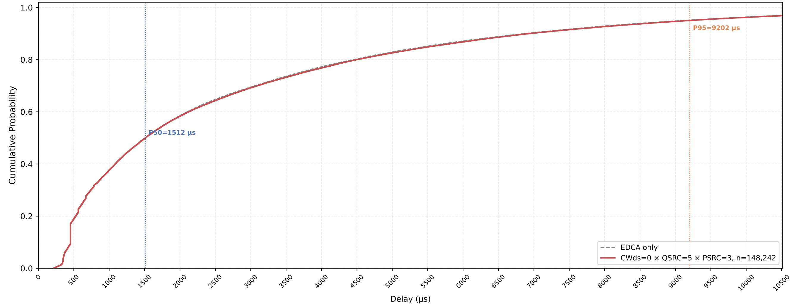
Legacy STA VO Delay CDF — CWds=0 × QSRC=5 × PSRC=3 nSta=30, nPedca=5, 1Mbps, avg of 10 runs
