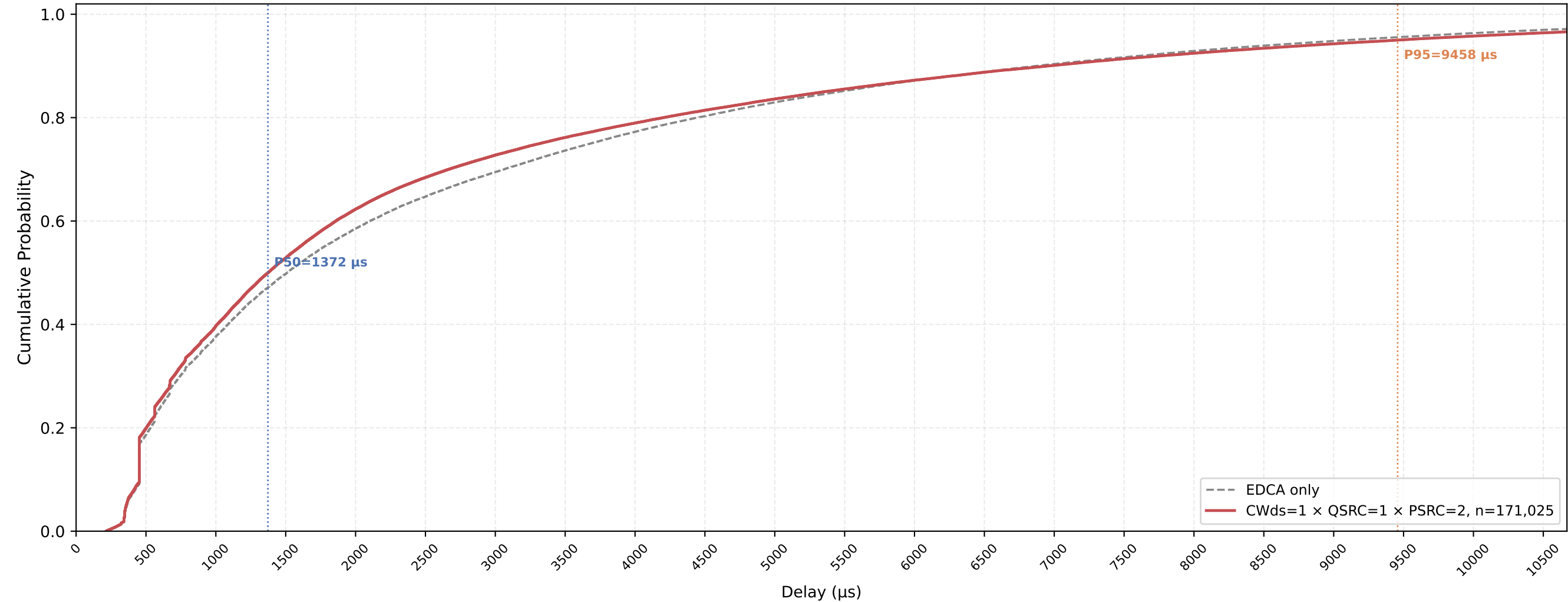
P-EDCA STA VO Delay CDF — CWds=1 × QSRC=1 × PSRC=2 nSta=30, nPedca=30, 1Mbps, avg of 10 runs
