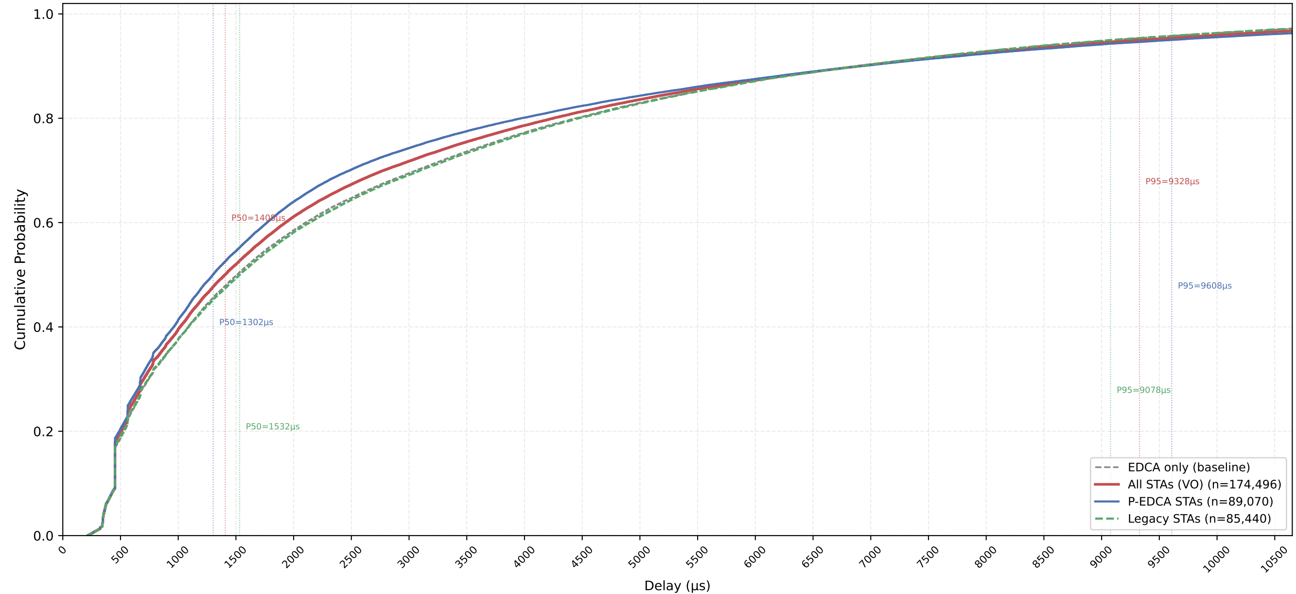
VO Delay CDF — P-EDCA / Legacy / All | CWds=1 × QSRC=1 × PSRC=3 nSta=30, nPedca=15/30, 1Mbps, avg of 10 runs
