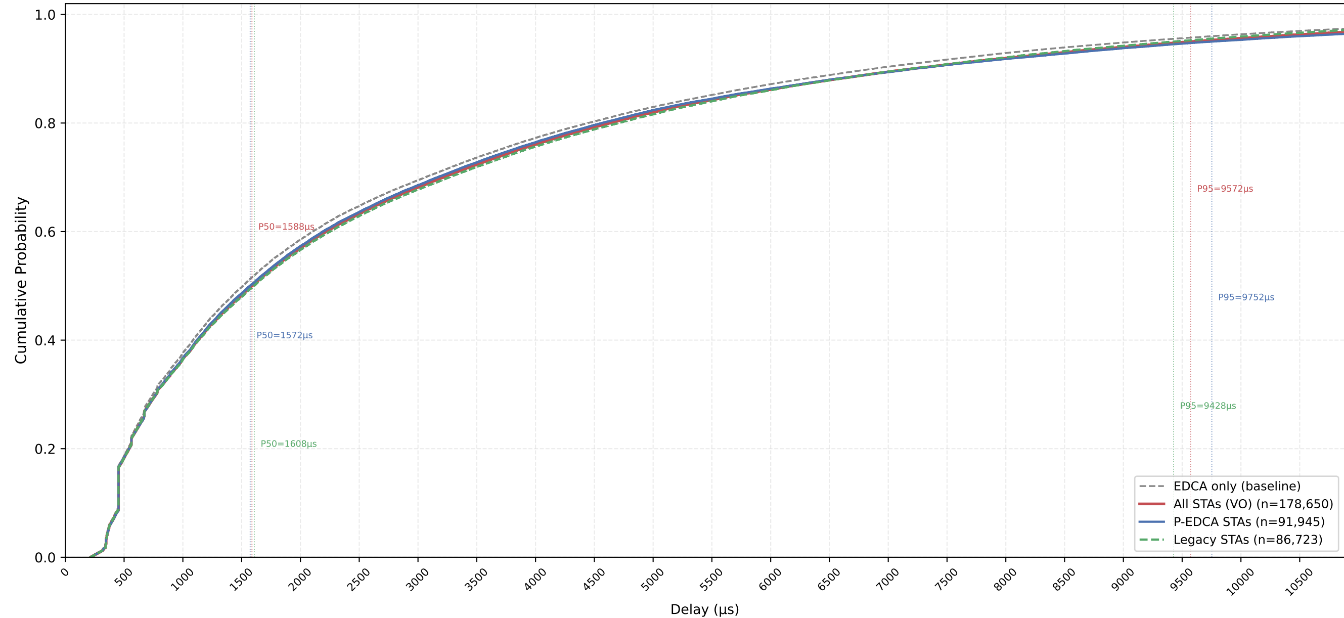
VO Delay CDF — P-EDCA / Legacy / All | CWds=1 × QSRC=2 × PSRC=1 nSta=30, nPedca=15/30, 1Mbps, avg of 10 runs
