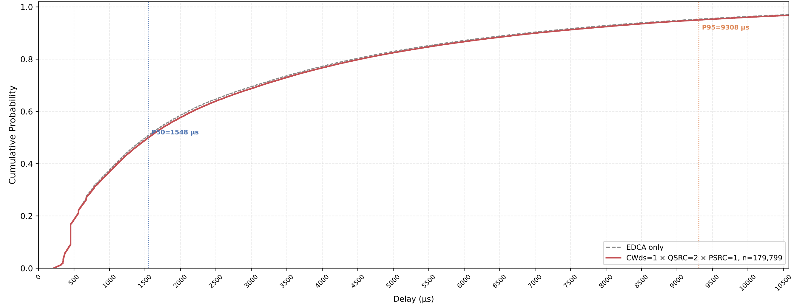
VO (all STAs) Delay CDF — CWds=1 × QSRC=2 × PSRC=1 nSta=30, nPedca=5, 1Mbps, avg of 10 runs
