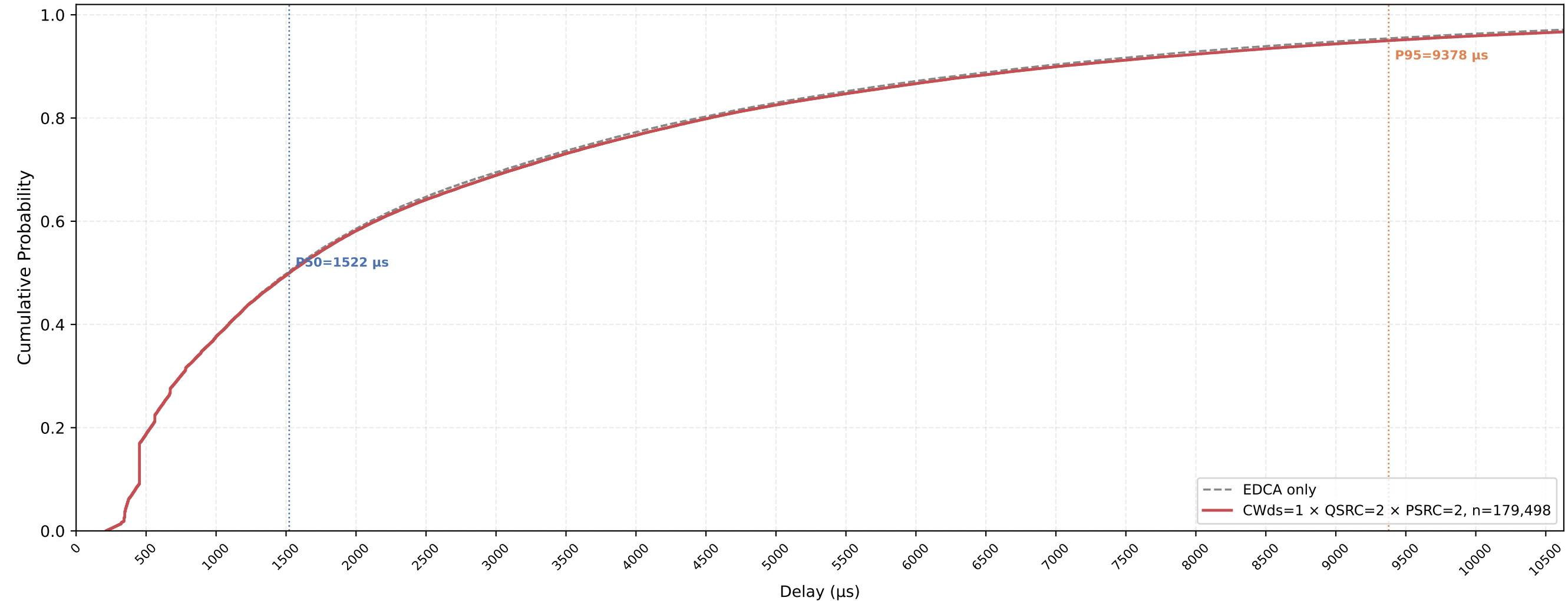
VO (all STAs) Delay CDF — CWds=1 × QSRC=2 × PSRC=2 nSta=30, nPedca=5, 1Mbps, avg of 10 runs
