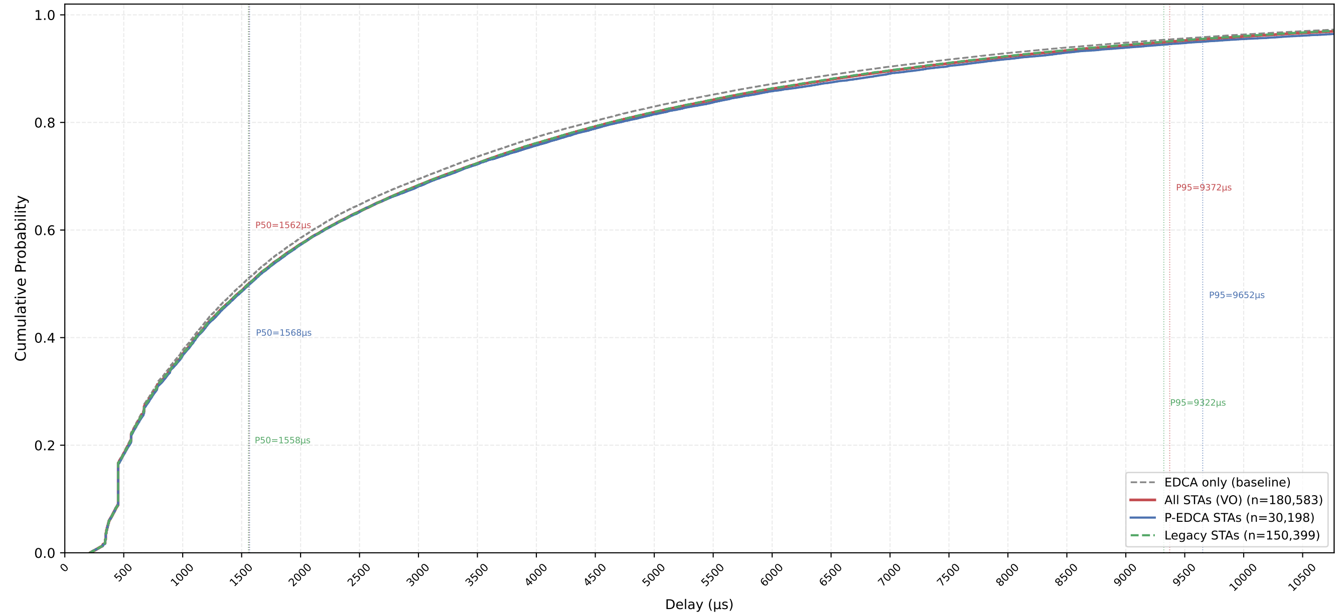
VO Delay CDF — P-EDCA / Legacy / All | CWds=1 × QSRC=5 × PSRC=1 nSta=30, nPedca=5/30, 1Mbps, avg of 10 runs
