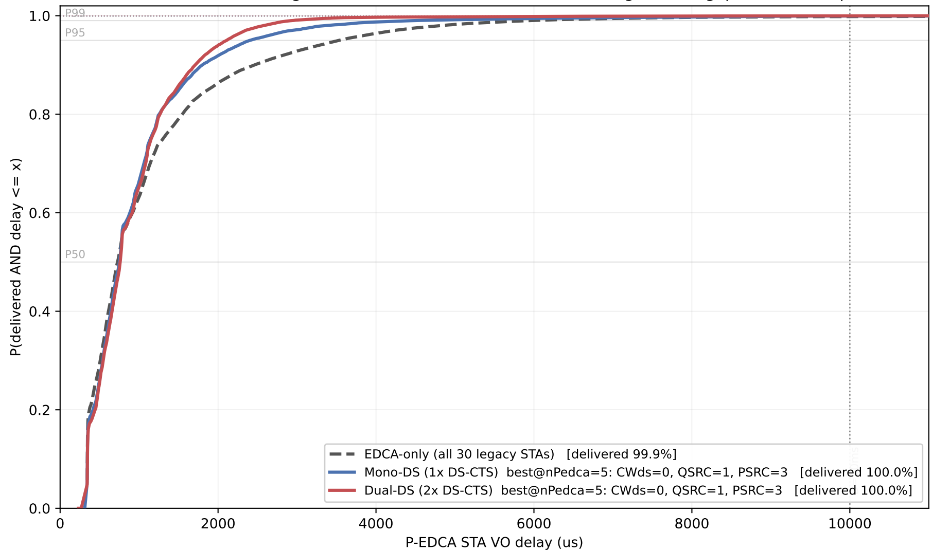
P-EDCA STA Delay CDF at Best Parameters (nPedca=5/30, nSta=30, 0.5Mbps)
