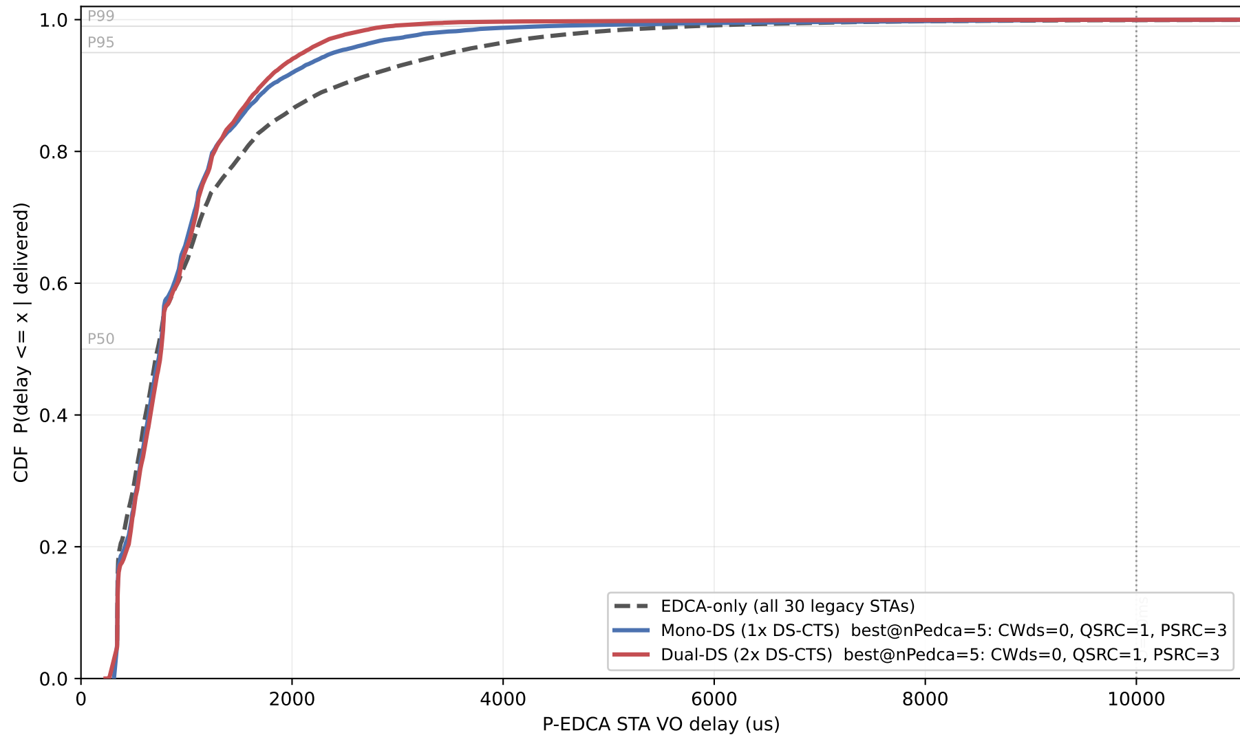
P-EDCA STA Delay CDF at Best Parameters (nPedca=5/30, nSta=30, 0.5Mbps) curves normalised to 1.0 — delay SHAPE only, loss not shown
