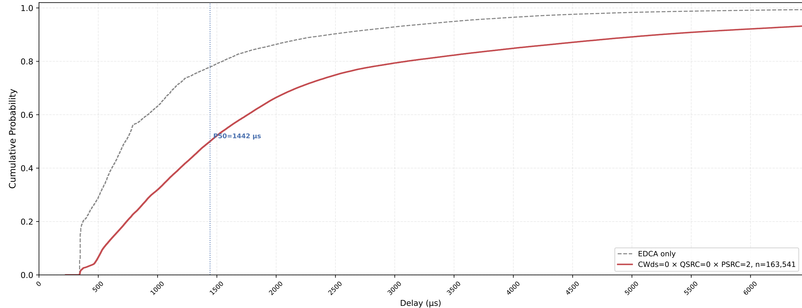
VO (all STAs) Delay CDF — CWds=0 × QSRC=0 × PSRC=2 nSta=30, nPedca=15, 0.5Mbps, avg of 10 runs
