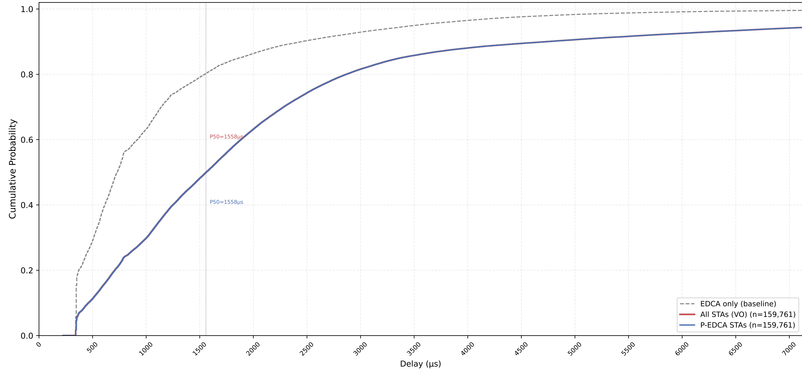
VO Delay CDF — P-EDCA / Legacy / All | CWds=0 × QSRC=1 × PSRC=2 nSta=30, nPedca=30/30, 0.5Mbps, avg of 10 runs
