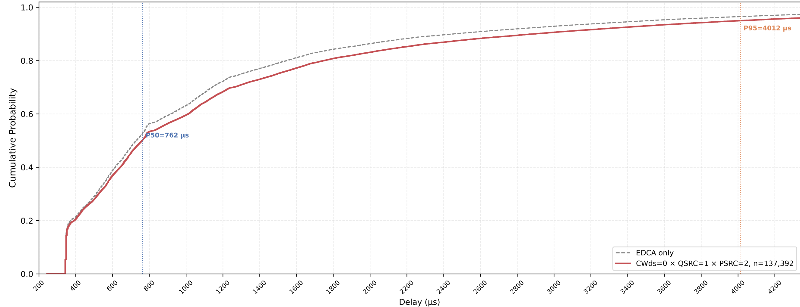
Legacy STA VO Delay CDF — CWds=0 × QSRC=1 × PSRC=2 nSta=30, nPedca=5, 0.5Mbps, avg of 10 runs
