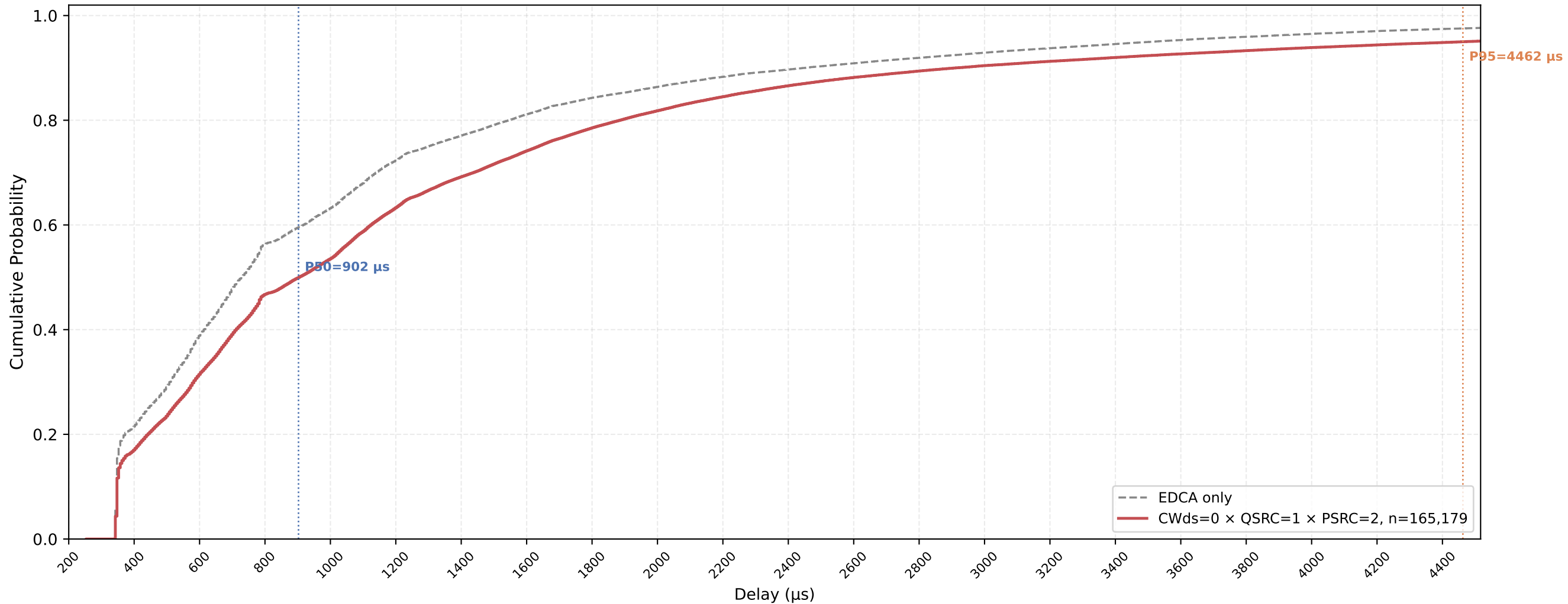
VO (all STAs) Delay CDF — CWds=0 × QSRC=1 × PSRC=2 nSta=30, nPedca=15, 0.5Mbps, avg of 10 runs
