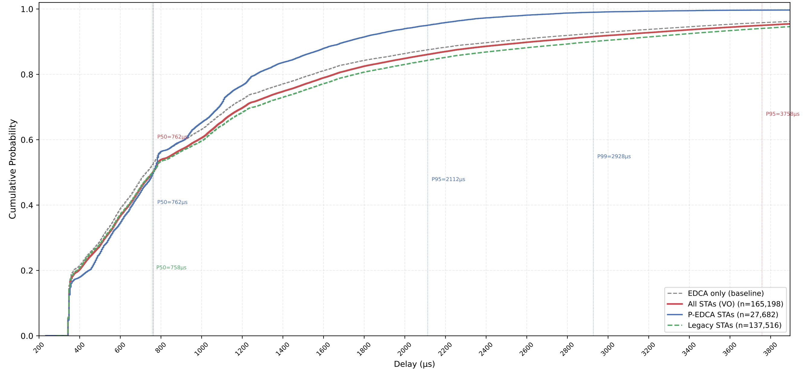
VO Delay CDF — P-EDCA / Legacy / All | CWds=0 × QSRC=1 × PSRC=3 nSta=30, nPedca=5/30, 0.5Mbps, avg of 10 runs
