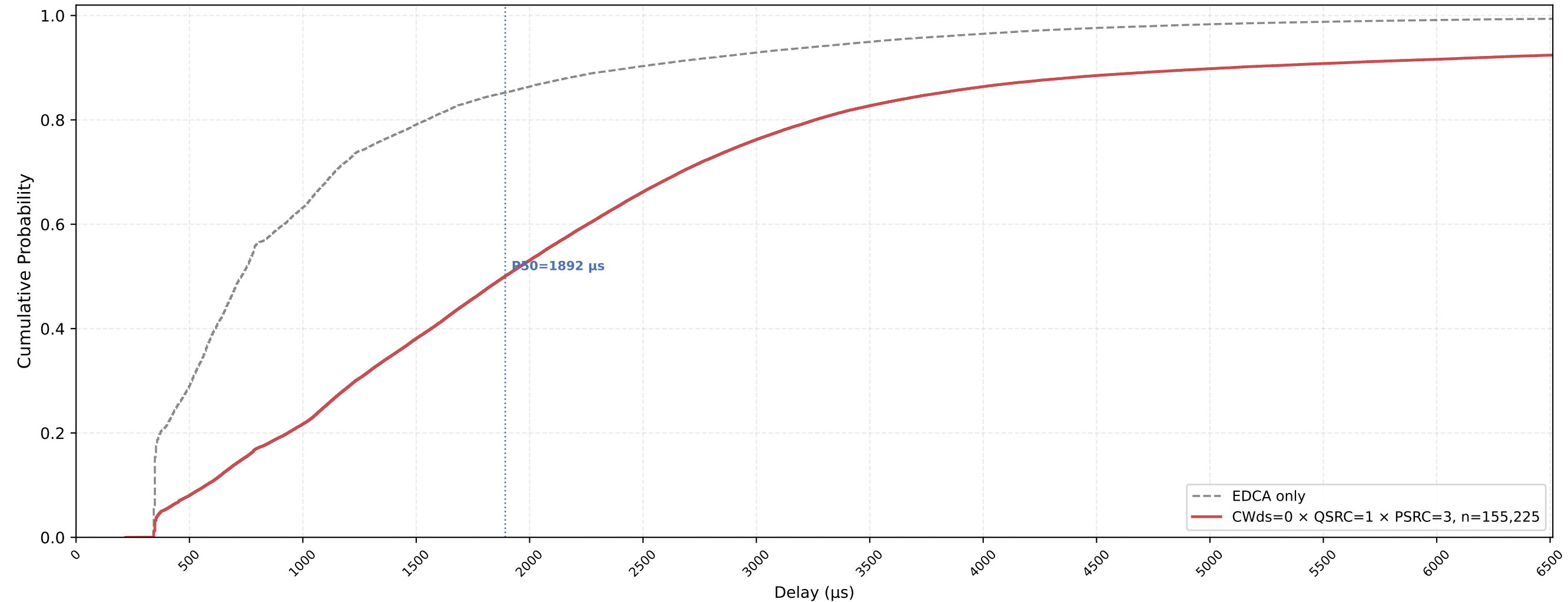
VO (all STAs) Delay CDF — CWds=0 × QSRC=1 × PSRC=3 nSta=30, nPedca=30, 0.5Mbps, avg of 10 runs
