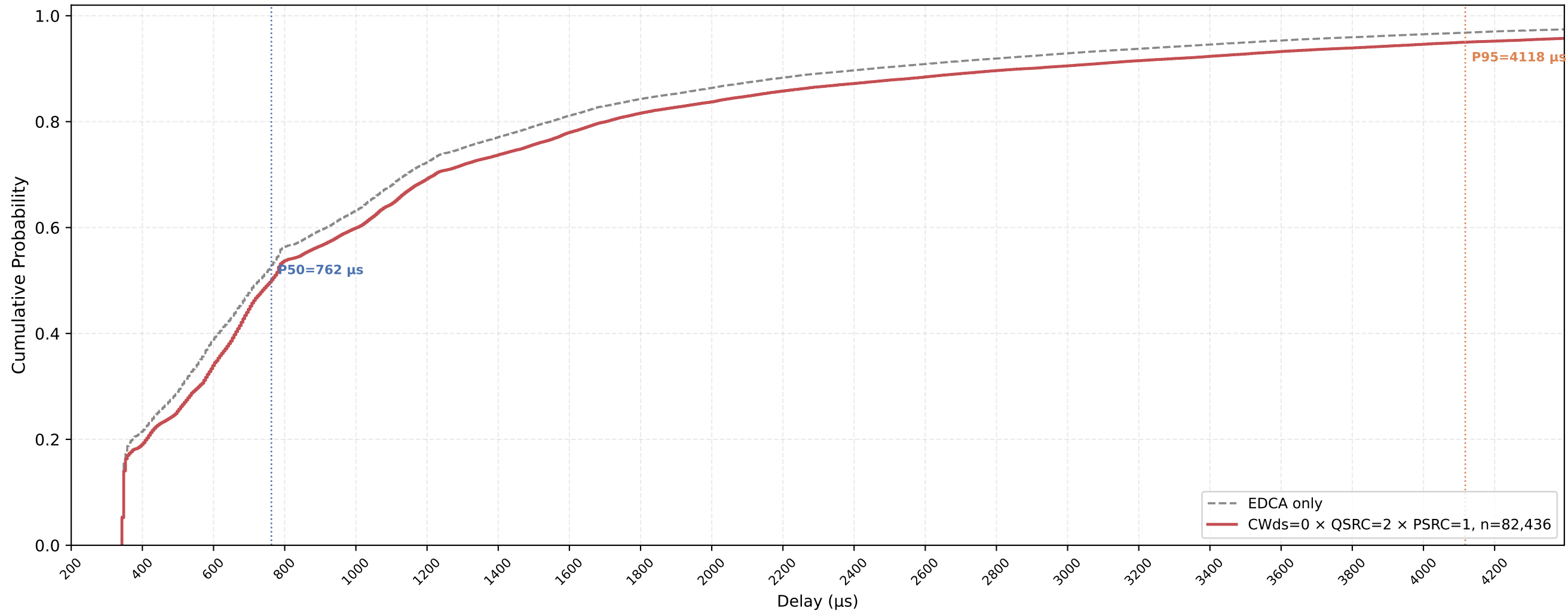
Legacy STA VO Delay CDF — CWds=0 × QSRC=2 × PSRC=1 nSta=30, nPedca=15, 0.5Mbps, avg of 10 runs
