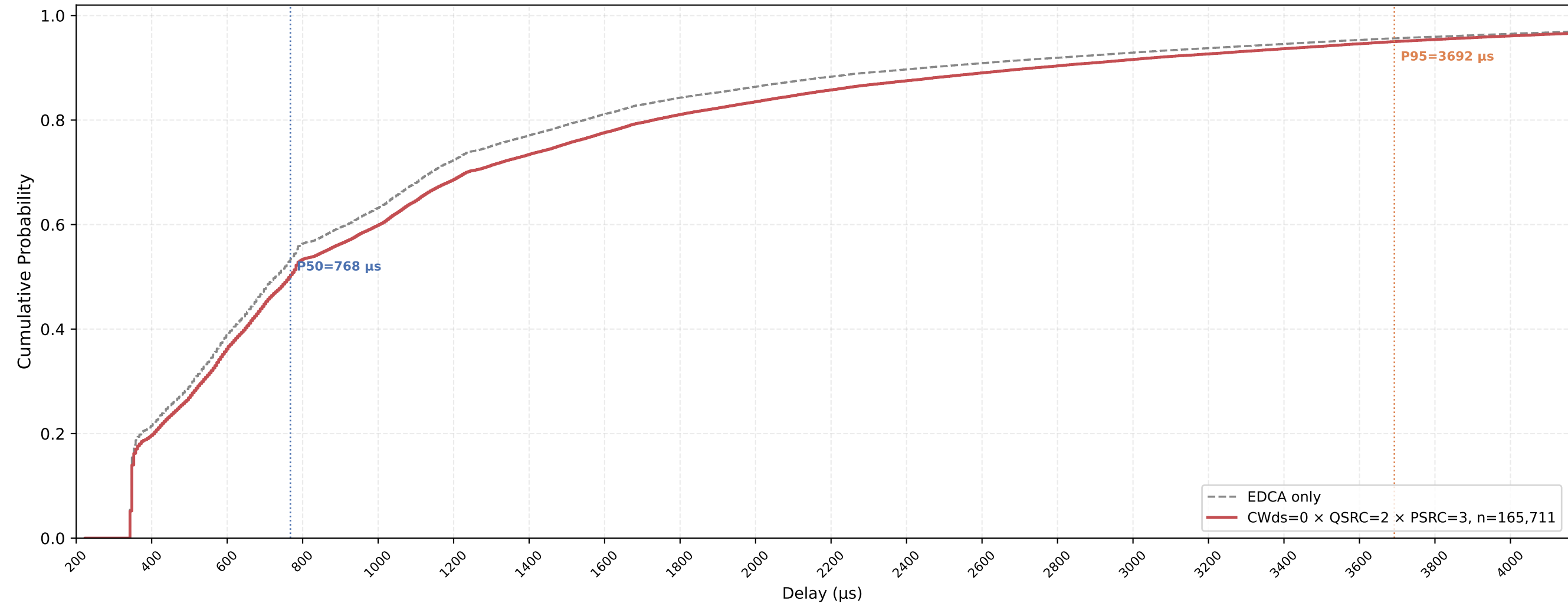
VO (all STAs) Delay CDF — CWds=0 × QSRC=2 × PSRC=3 nSta=30, nPedca=15, 0.5Mbps, avg of 10 runs
