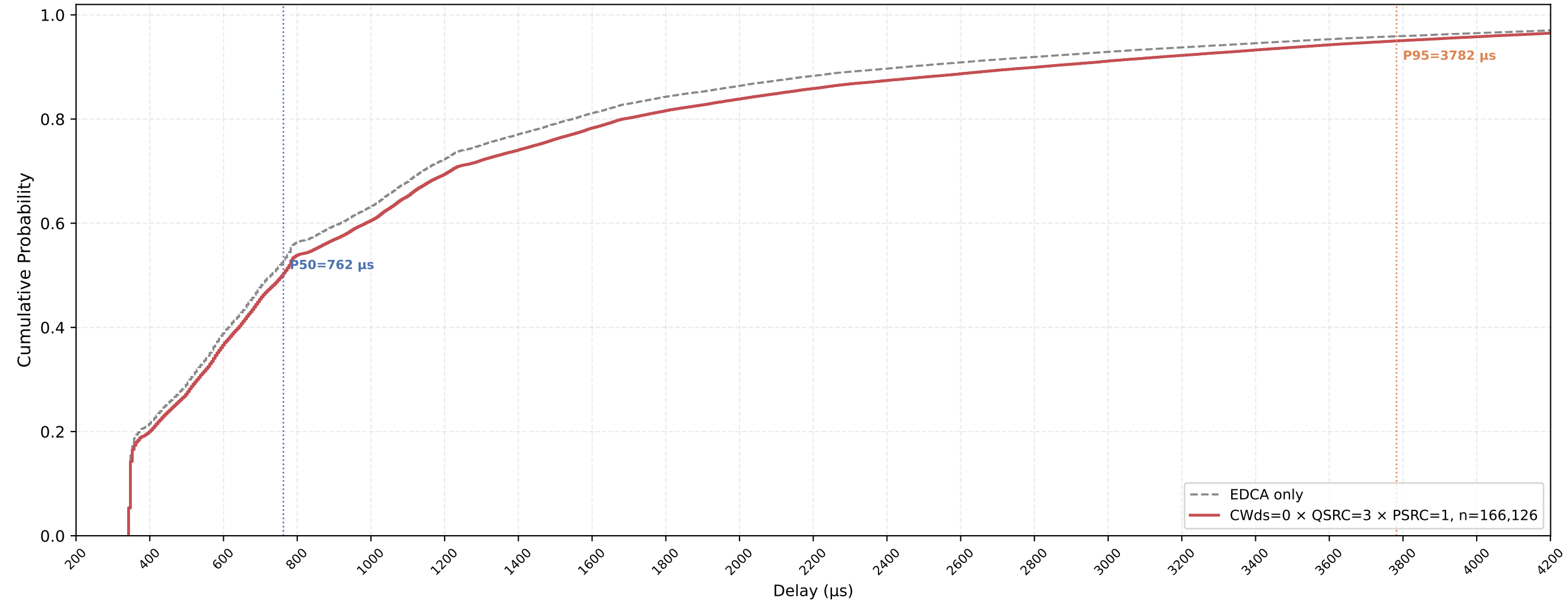
P-EDCA STA VO Delay CDF — CWds=0 × QSRC=3 × PSRC=1 nSta=30, nPedca=30, 0.5Mbps, avg of 10 runs
