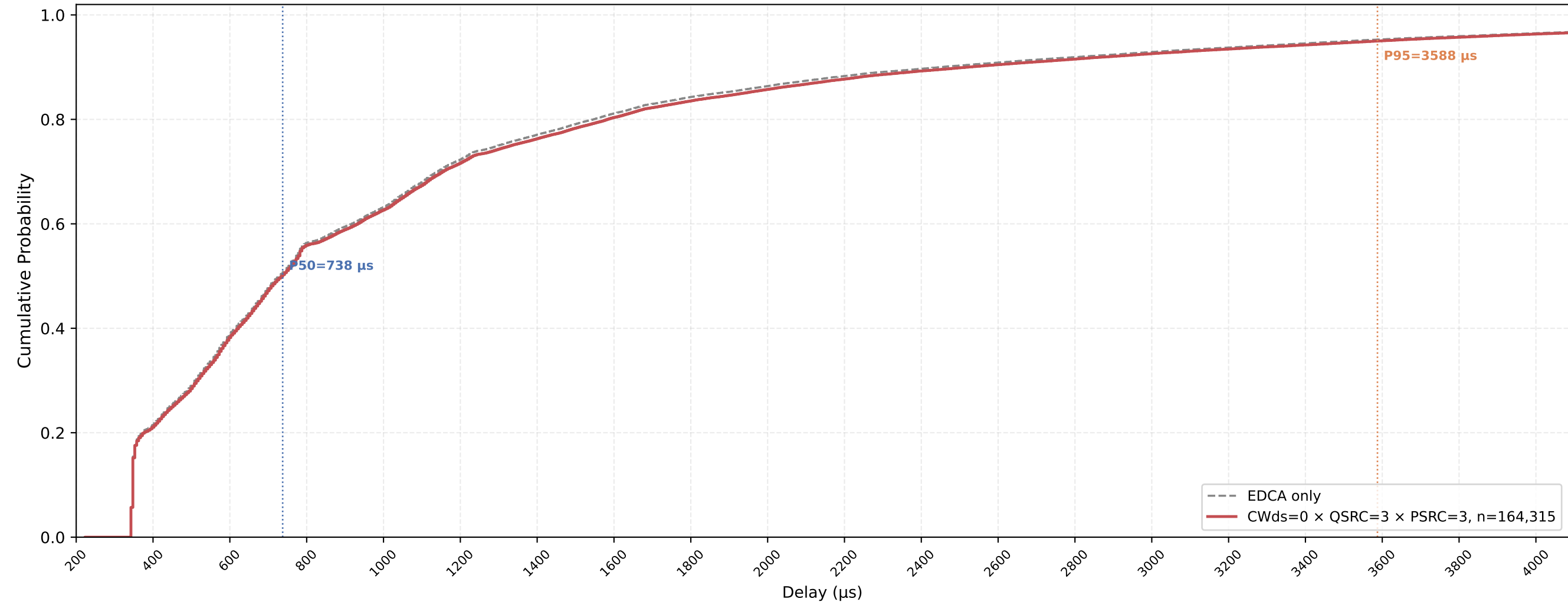
VO (all STAs) Delay CDF — CWds=0 × QSRC=3 × PSRC=3 nSta=30, nPedca=5, 0.5Mbps, avg of 10 runs
