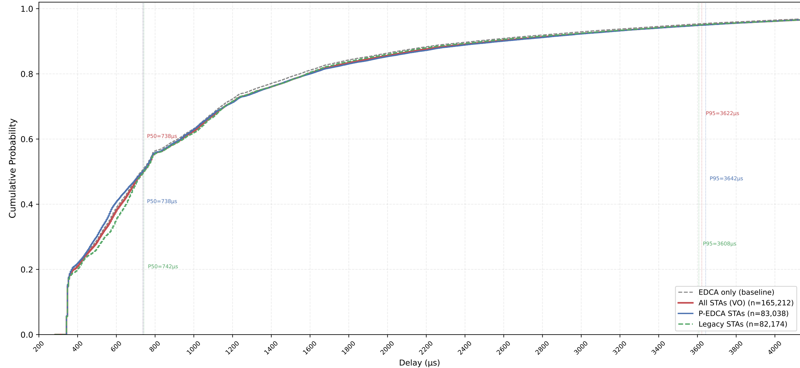
VO Delay CDF — P-EDCA / Legacy / All | CWds=0 × QSRC=4 × PSRC=1 nSta=30, nPedca=15/30, 0.5Mbps, avg of 10 runs
